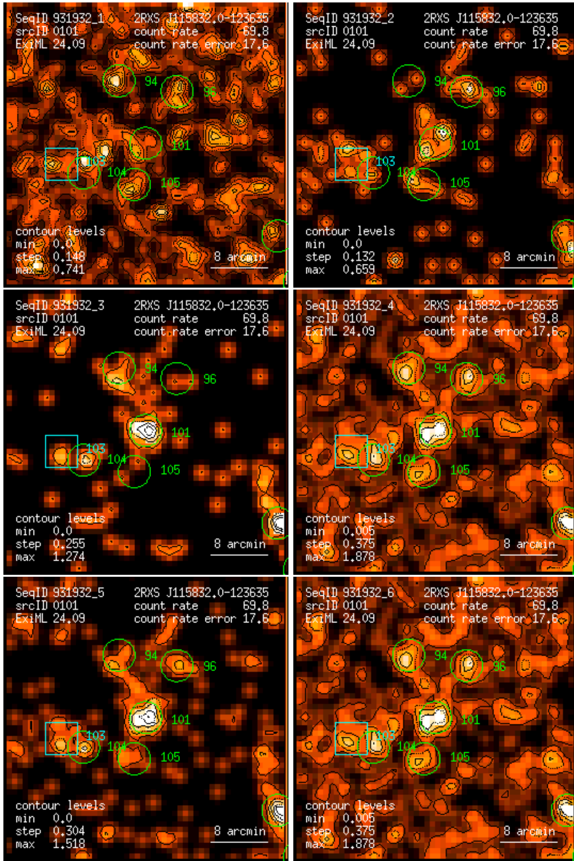
Figure 101: RASS 931932: detection 0101: band rate images, Gaussian filter: (1) PSPC channels 11 – 41, (2) 52 – 90, (3) 91 – 201, (4) 11 – 235, (5) 52 – 201, (6) 11 – 201. Broad band rates in counts/ks. Band rate contour levels in counts/ks/arcmin 2 .
