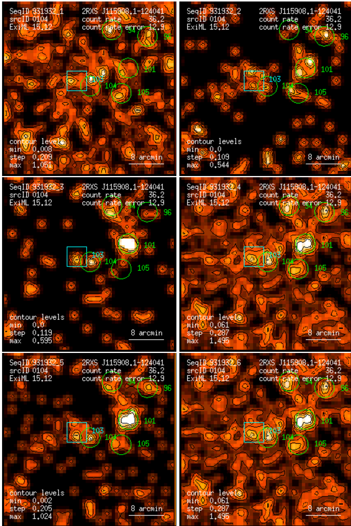
Figure 104: RASS 931932: detection 0104: band rate images, Gaussian filter: (1) PSPC channels 11 – 41, (2) 52 – 90, (3) 91 – 201, (4) 11 – 235, (5) 52 – 201, (6) 11 – 201. Broad band rates in counts/ks. Band rate contour levels in counts/ks/arcmin 2 .
