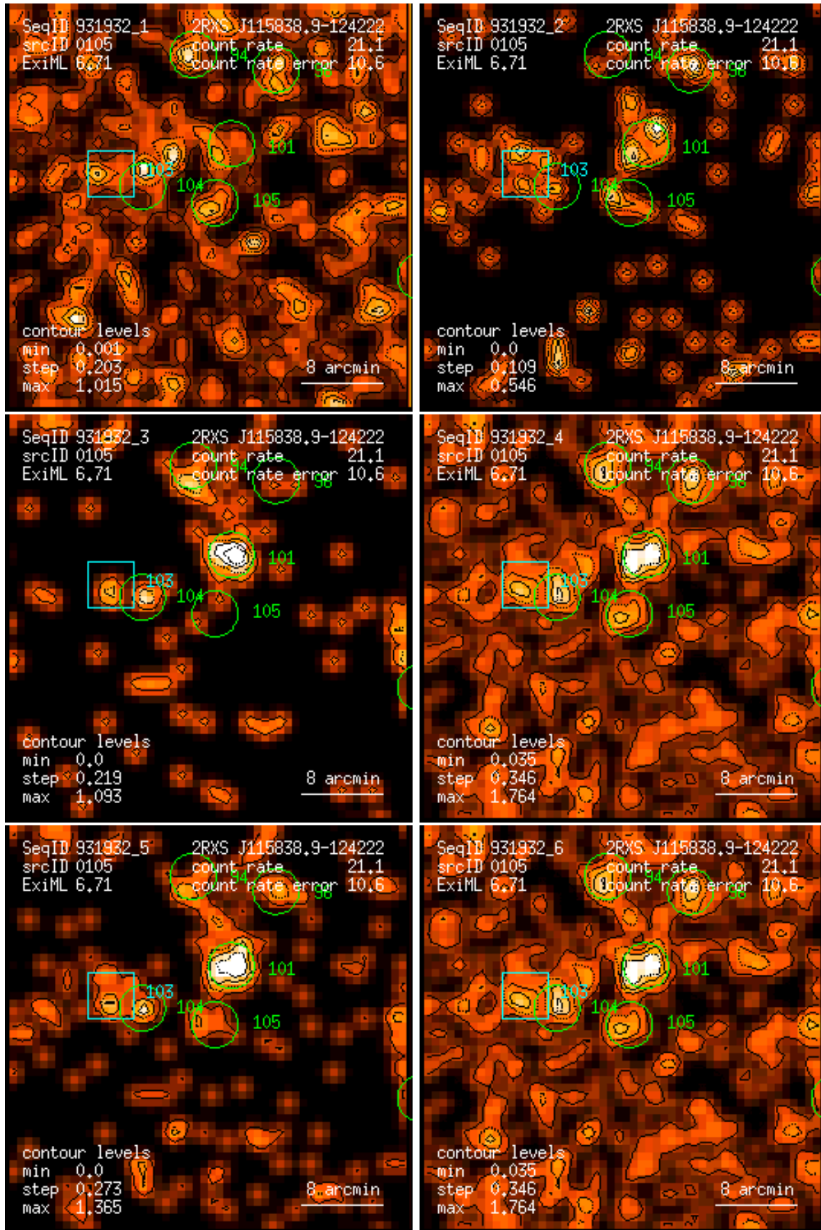
Figure 105: RASS 931932: detection 0105: band rate images, Gaussian filter: (1) PSPC channels 11 – 41, (2) 52 – 90, (3) 91 – 201, (4) 11 – 235, (5) 52 – 201, (6) 11 – 201. Broad band rates in counts/ks. Band rate contour levels in counts/ks/arcmin 2 .
