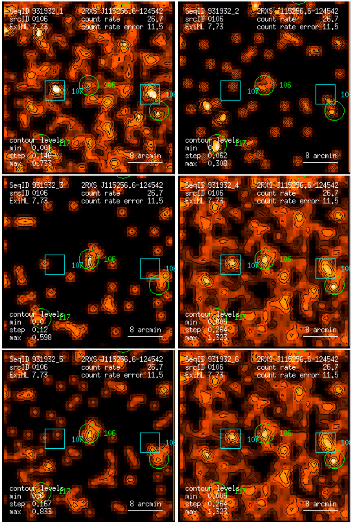
Figure 106: RASS 931932: detection 0106: band rate images, Gaussian filter: (1) PSPC channels 11 – 41, (2) 52 – 90, (3) 91 – 201, (4) 11 – 235, (5) 52 – 201, (6) 11 – 201. Broad band rates in counts/ks. Band rate contour levels in counts/ks/arcmin 2 .
