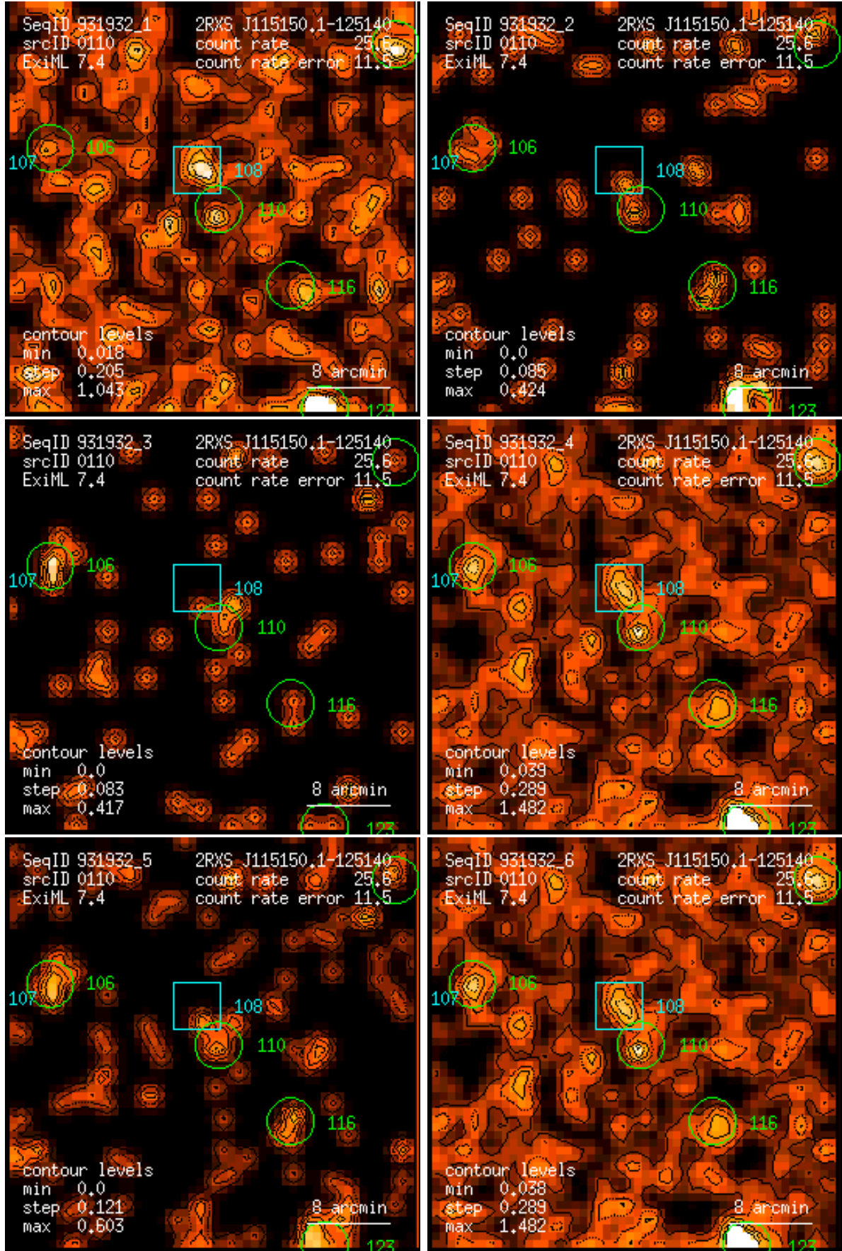
Figure 110: RASS 931932: detection 0110: band rate images, Gaussian filter: (1) PSPC channels 11 – 41, (2) 52 – 90, (3) 91 – 201, (4) 11 – 235, (5) 52 – 201, (6) 11 – 201. Broad band rates in counts/ks. Band rate contour levels in counts/ks/arcmin 2 .
