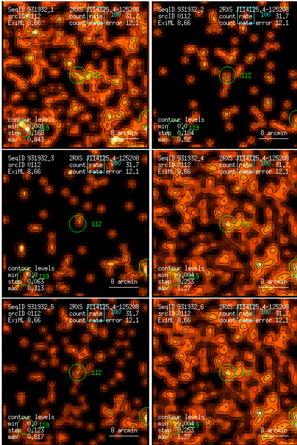
Figure 112: RASS 931932: detection 0112: band rate images, Gaussian filter: (1) PSPC channels 11 – 41, (2) 52 – 90, (3) 91 – 201, (4) 11 – 235, (5) 52 – 201, (6) 11 – 201. Broad band rates in counts/ks. Band rate contour levels in counts/ks/arcmin 2 .
