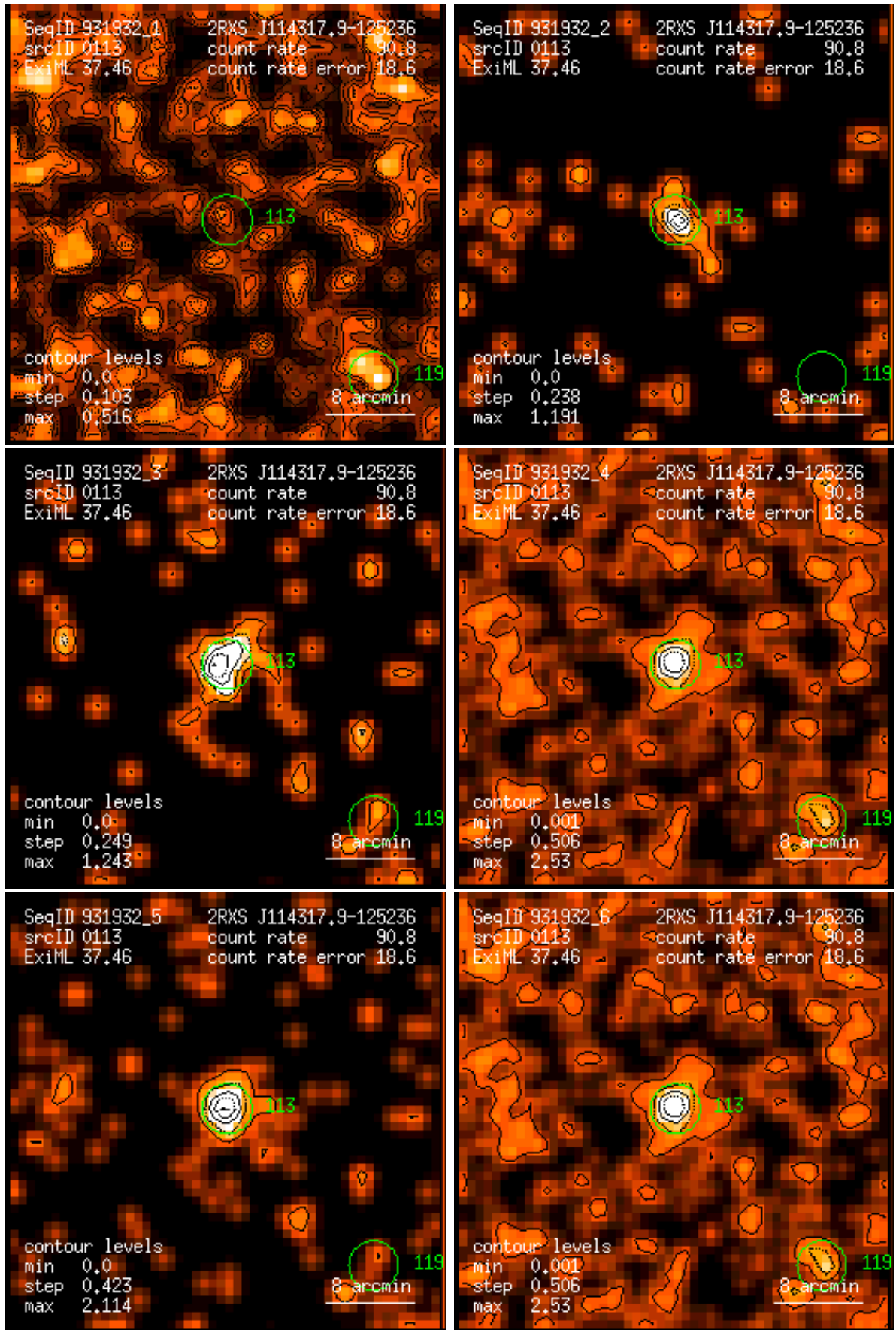
Figure 113: RASS 931932: detection 0113: band rate images, Gaussian filter: (1) PSPC channels 11 – 41, (2) 52 – 90, (3) 91 – 201, (4) 11 – 235, (5) 52 – 201, (6) 11 – 201. Broad band rates in counts/ks. Band rate contour levels in counts/ks/arcmin 2 .
