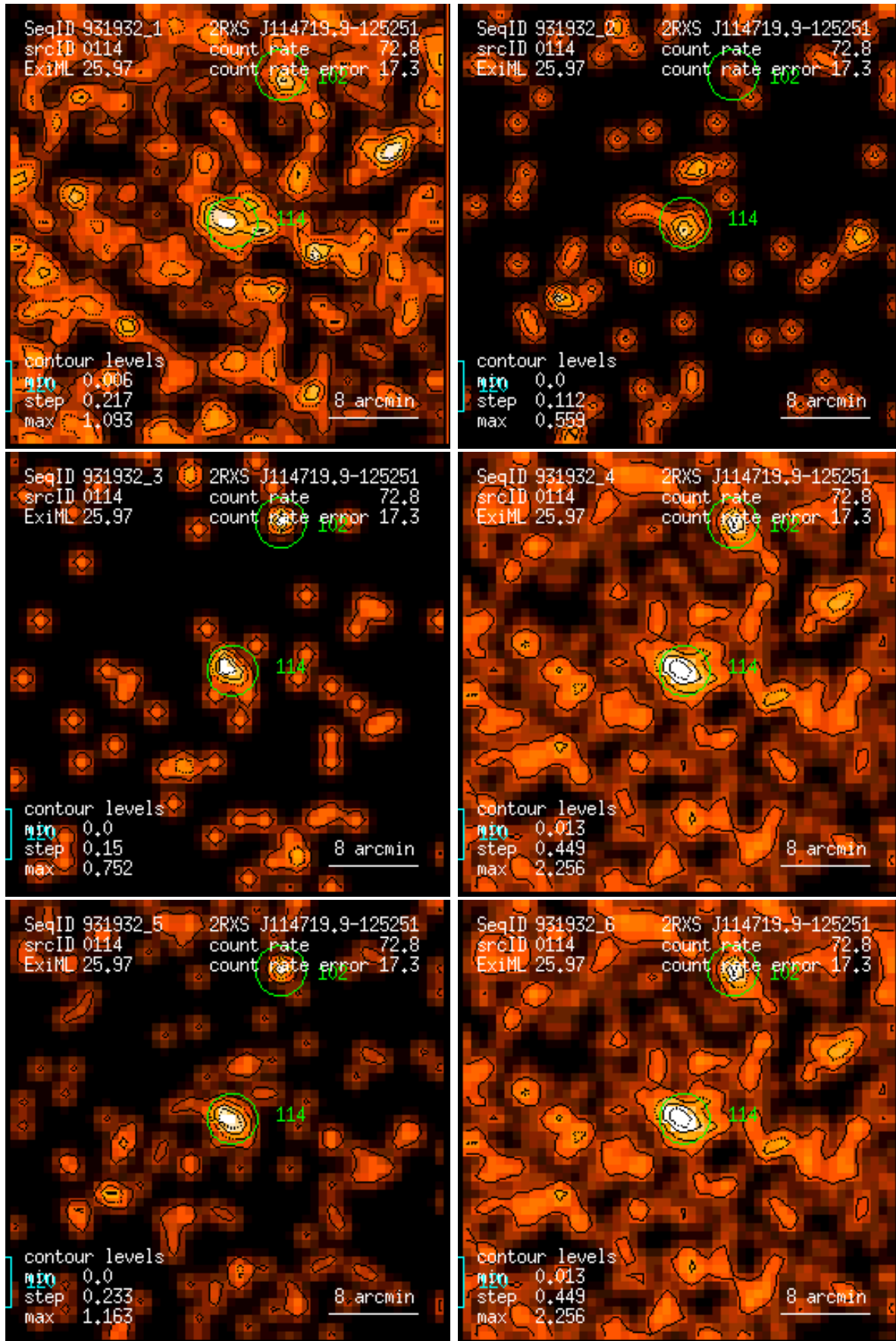
Figure 114: RASS 931932: detection 0114: band rate images, Gaussian filter: (1) PSPC channels 11 – 41, (2) 52 – 90, (3) 91 – 201, (4) 11 – 235, (5) 52 – 201, (6) 11 – 201. Broad band rates in counts/ks. Band rate contour levels in counts/ks/arcmin 2 .
