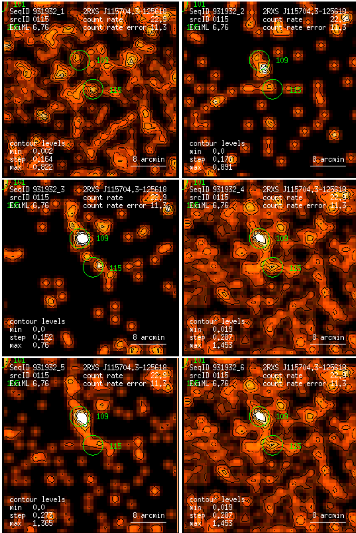
Figure 115: RASS 931932: detection 0115: band rate images, Gaussian filter: (1) PSPC channels 11 – 41, (2) 52 – 90, (3) 91 – 201, (4) 11 – 235, (5) 52 – 201, (6) 11 – 201. Broad band rates in counts/ks. Band rate contour levels in counts/ks/arcmin 2 .
