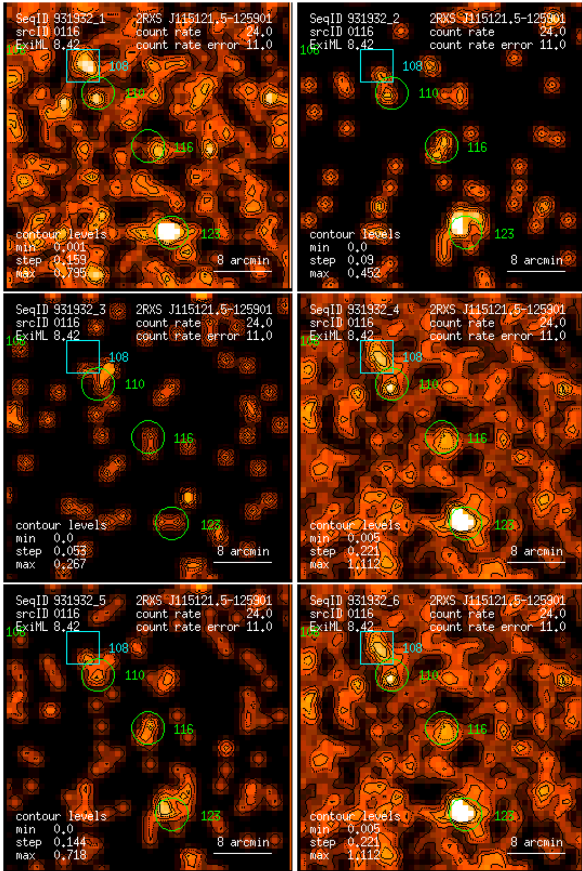
Figure 116: RASS 931932: detection 0116: band rate images, Gaussian filter: (1) PSPC channels 11 – 41, (2) 52 – 90, (3) 91 – 201, (4) 11 – 235, (5) 52 – 201, (6) 11 – 201. Broad band rates in counts/ks. Band rate contour levels in counts/ks/arcmin 2 .
