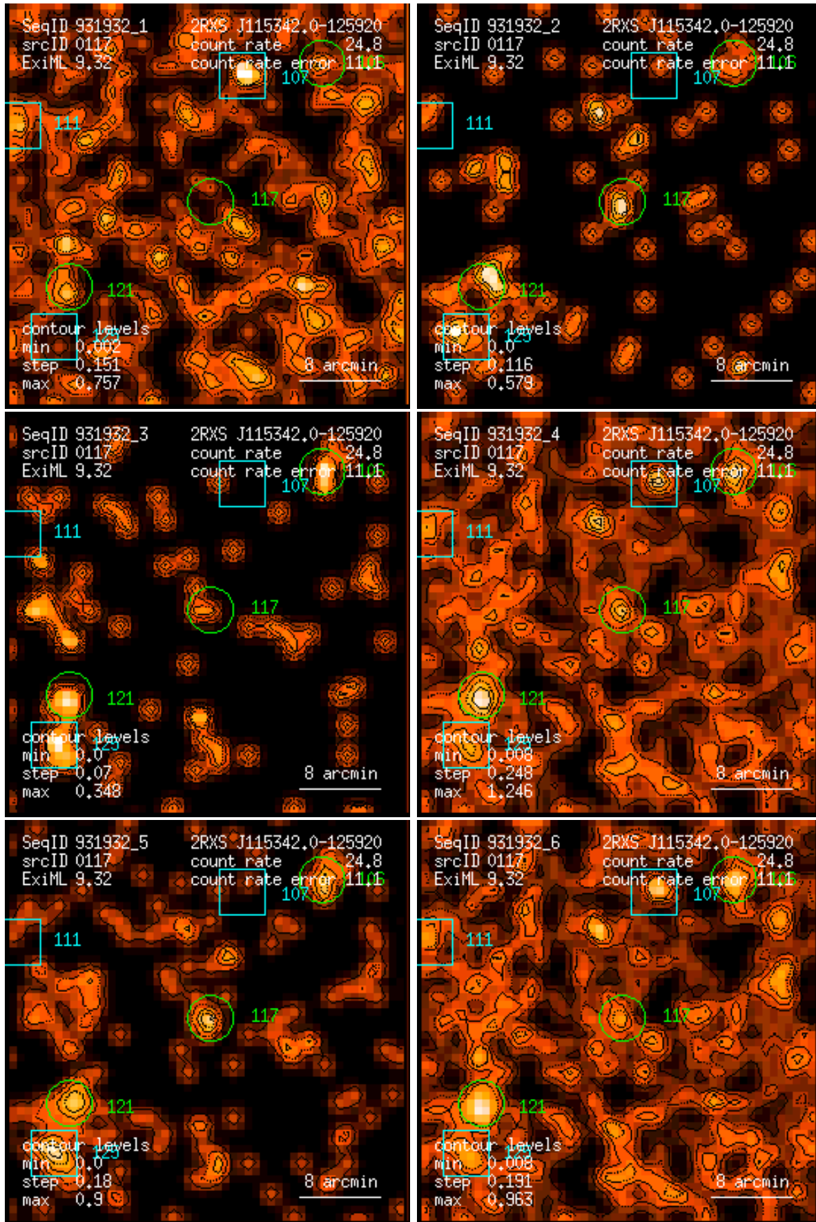
Figure 117: RASS 931932: detection 0117: band rate images, Gaussian filter: (1) PSPC channels 11 – 41, (2) 52 – 90, (3) 91 – 201, (4) 11 – 235, (5) 52 – 201, (6) 11 – 201. Broad band rates in counts/ks. Band rate contour levels in counts/ks/arcmin 2 .
