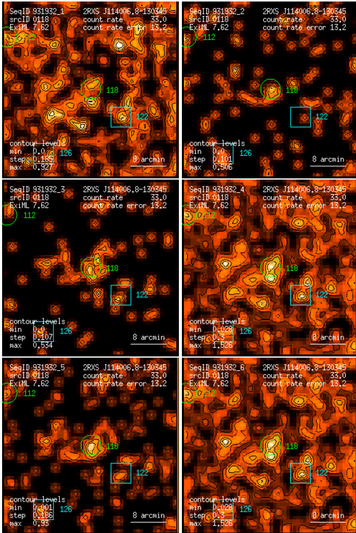
Figure 118: RASS 931932: detection 0118: band rate images, Gaussian filter: (1) PSPC channels 11 – 41, (2) 52 – 90, (3) 91 – 201, (4) 11 – 235, (5) 52 – 201, (6) 11 – 201. Broad band rates in counts/ks. Band rate contour levels in counts/ks/arcmin 2 .
