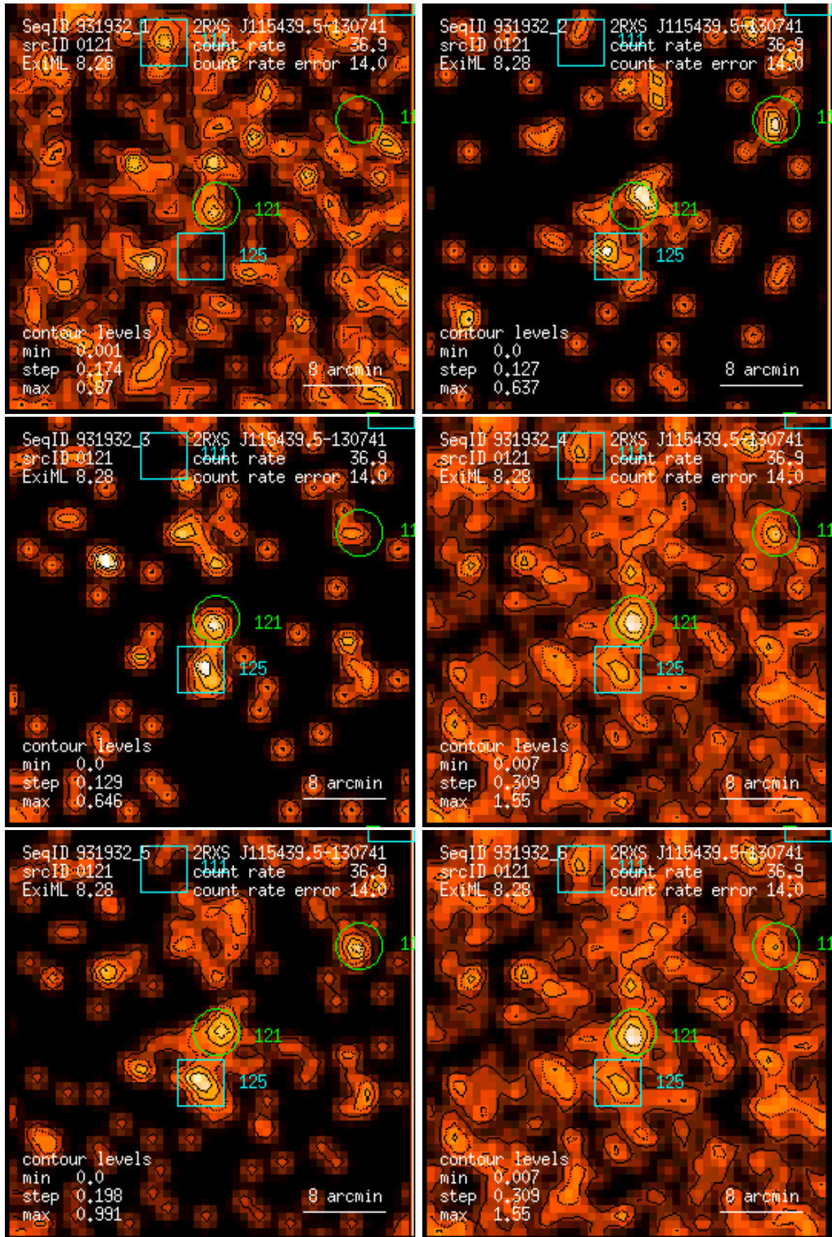
Figure 121: RASS 931932: detection 0121: band rate images, Gaussian filter: (1) PSPC channels 11 – 41, (2) 52 – 90, (3) 91 – 201, (4) 11 – 235, (5) 52 – 201, (6) 11 – 201. Broad band rates in counts/ks. Band rate contour levels in counts/ks/arcmin 2 .
