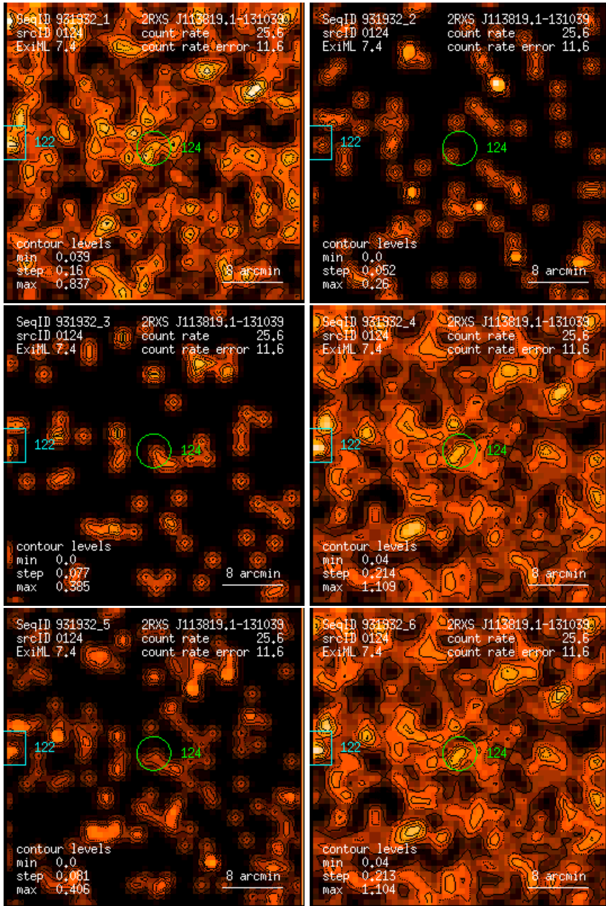
Figure 124: RASS 931932: detection 0124: band rate images, Gaussian filter: (1) PSPC channels 11 – 41, (2) 52 – 90, (3) 91 – 201, (4) 11 – 235, (5) 52 – 201, (6) 11 – 201. Broad band rates in counts/ks. Band rate contour levels in counts/ks/arcmin 2 .
