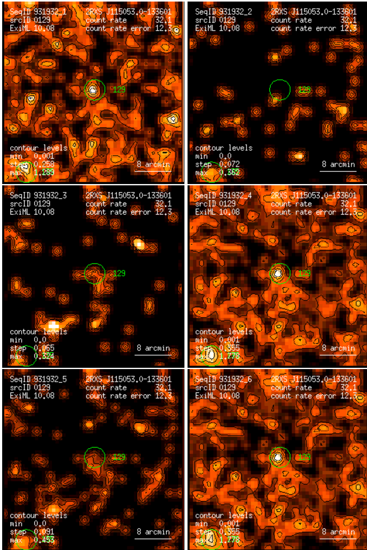
Figure 129: RASS 931932: detection 0129: band rate images, Gaussian filter: (1) PSPC channels 11 – 41, (2) 52 – 90, (3) 91 – 201, (4) 11 – 235, (5) 52 – 201, (6) 11 – 201. Broad band rates in counts/ks. Band rate contour levels in counts/ks/arcmin 2 .
