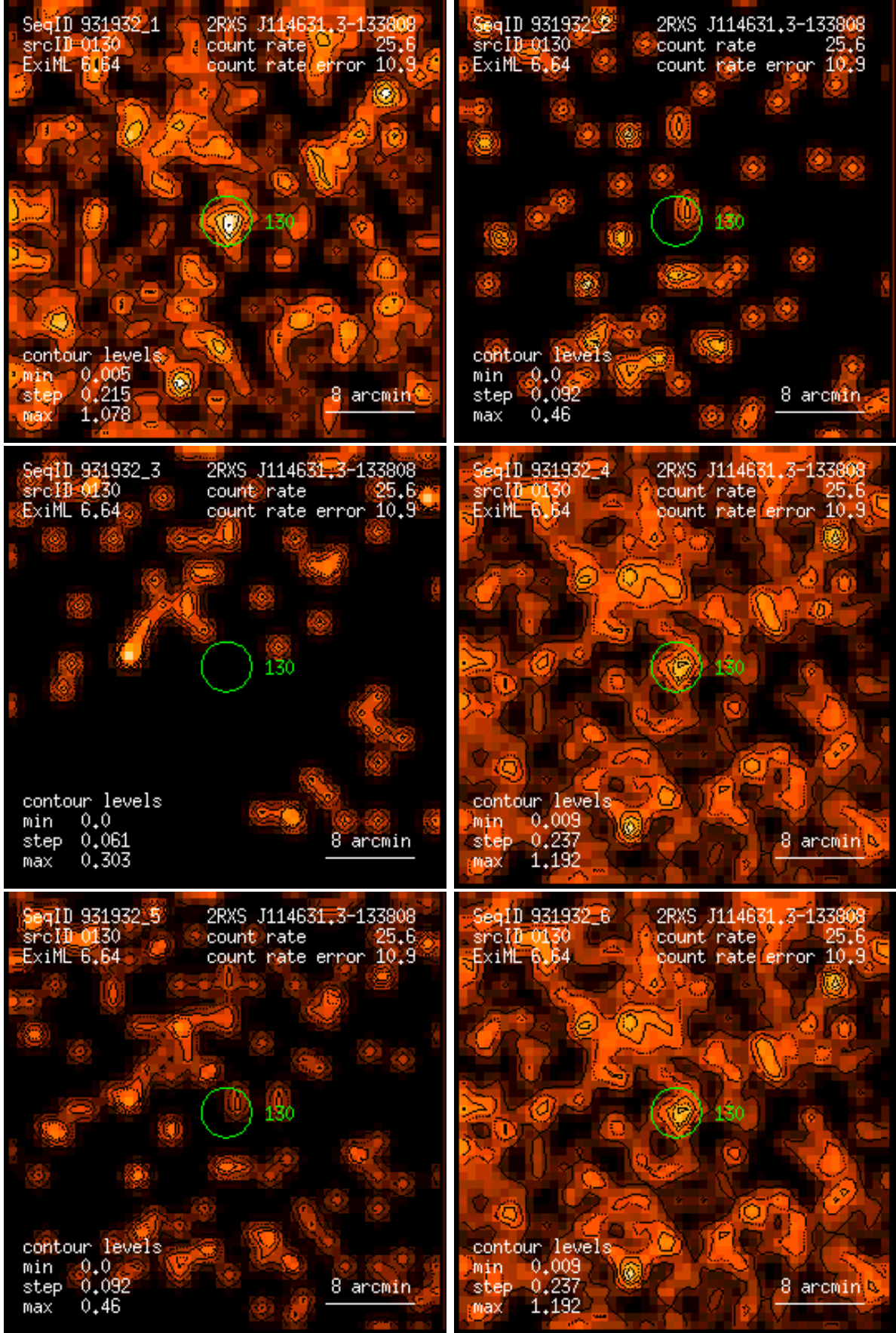
Figure 130: RASS 931932: detection 0130: band rate images, Gaussian filter: (1) PSPC channels 11 – 41, (2) 52 – 90, (3) 91 – 201, (4) 11 – 235, (5) 52 – 201, (6) 11 – 201. Broad band rates in counts/ks. Band rate contour levels in counts/ks/arcmin 2 .
