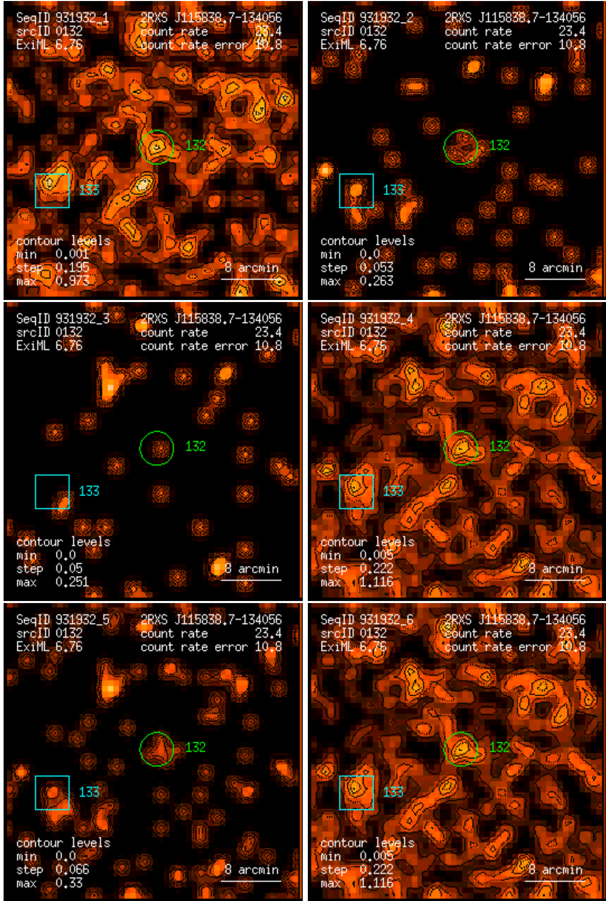
Figure 132: RASS 931932: detection 0132: band rate images, Gaussian filter: (1) PSPC channels 11 – 41, (2) 52 – 90, (3) 91 – 201, (4) 11 – 235, (5) 52 – 201, (6) 11 – 201. Broad band rates in counts/ks. Band rate contour levels in counts/ks/arcmin 2 .
