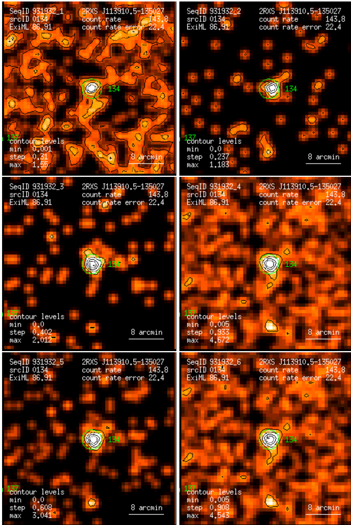
Figure 134: RASS 931932: detection 0134: band rate images, Gaussian filter: (1) PSPC channels 11 – 41, (2) 52 – 90, (3) 91 – 201, (4) 11 – 235, (5) 52 – 201, (6) 11 – 201. Broad band rates in counts/ks. Band rate contour levels in counts/ks/arcmin 2 .
