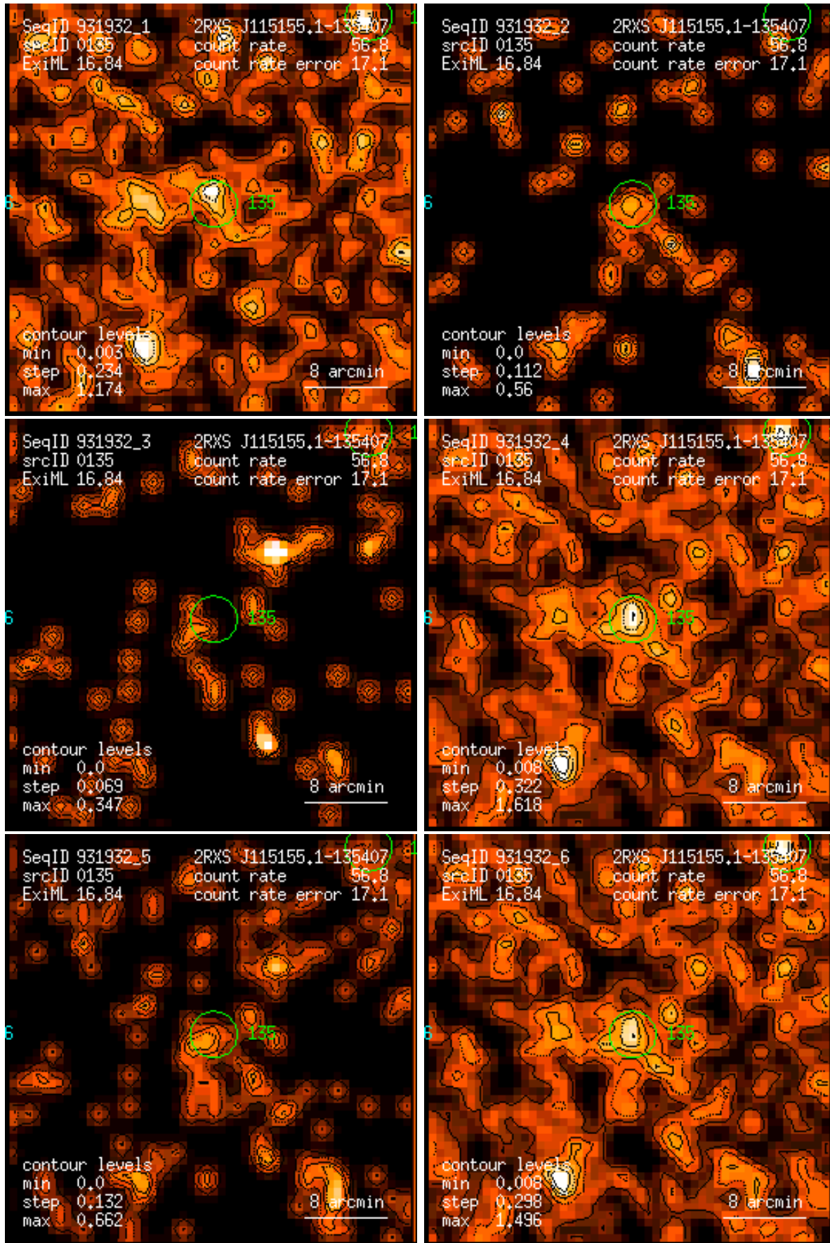
Figure 135: RASS 931932: detection 0135: band rate images, Gaussian filter: (1) PSPC channels 11 – 41, (2) 52 – 90, (3) 91 – 201, (4) 11 – 235, (5) 52 – 201, (6) 11 – 201. Broad band rates in counts/ks. Band rate contour levels in counts/ks/arcmin 2 .
