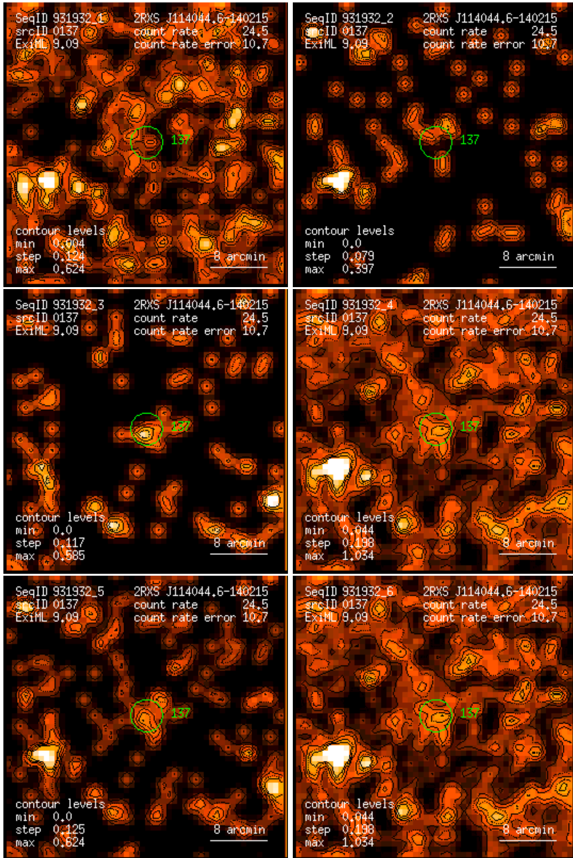
Figure 137: RASS 931932: detection 0137: band rate images, Gaussian filter: (1) PSPC channels 11 – 41, (2) 52 – 90, (3) 91 – 201, (4) 11 – 235, (5) 52 – 201, (6) 11 – 201. Broad band rates in counts/ks. Band rate contour levels in counts/ks/arcmin 2 .
