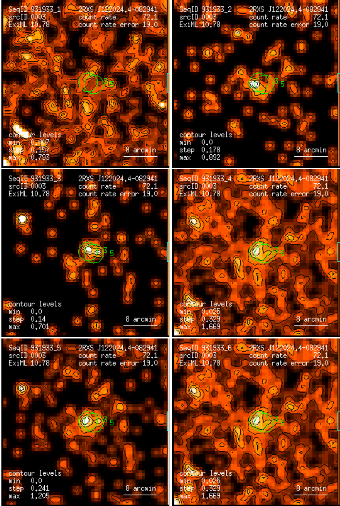
Figure 3: RASS 931933: detection 0003: band rate images, Gaussian filter: (1) PSPC channels 11 – 41, (2) 52 – 90, (3) 91 – 201, (4) 11 – 235, (5) 52 – 201, (6) 11 – 201. Broad band rates in counts/ks. Band rate contour levels in counts/ks/arcmin 2 .
