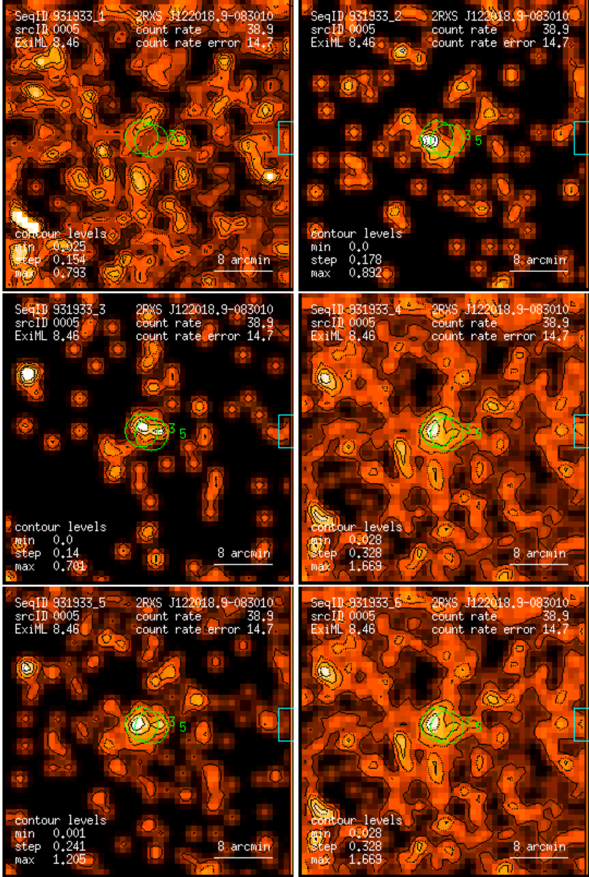
Figure 5: RASS 931933: detection 0005: band rate images, Gaussian filter: (1) PSPC channels 11 – 41, (2) 52 – 90, (3) 91 – 201, (4) 11 – 235, (5) 52 – 201, (6) 11 – 201. Broad band rates in counts/ks. Band rate contour levels in counts/ks/arcmin 2 .
