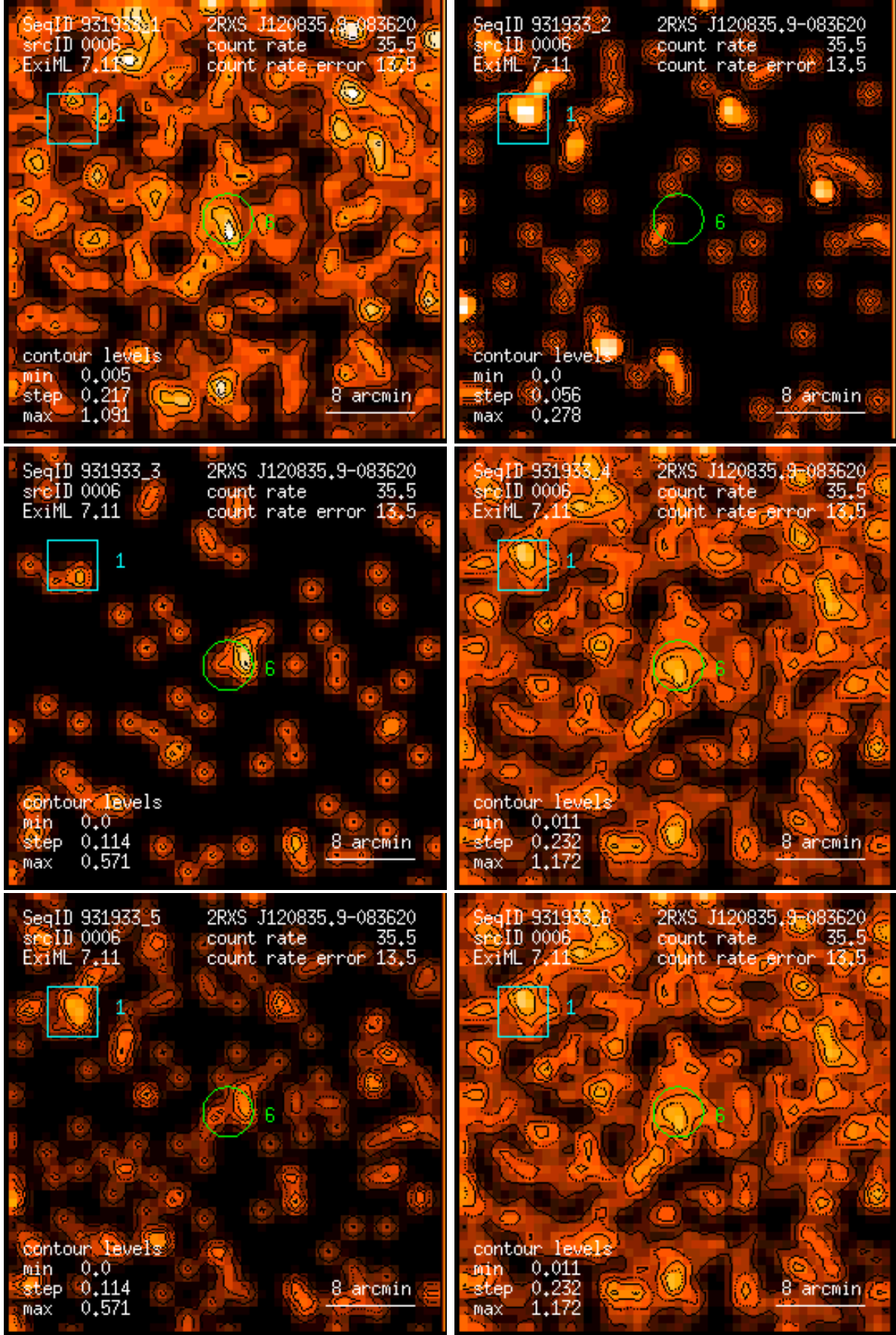
Figure 6: RASS 931933: detection 0006: band rate images, Gaussian filter: (1) PSPC channels 11 – 41, (2) 52 – 90, (3) 91 – 201, (4) 11 – 235, (5) 52 – 201, (6) 11 – 201. Broad band rates in counts/ks. Band rate contour levels in counts/ks/arcmin 2 .
