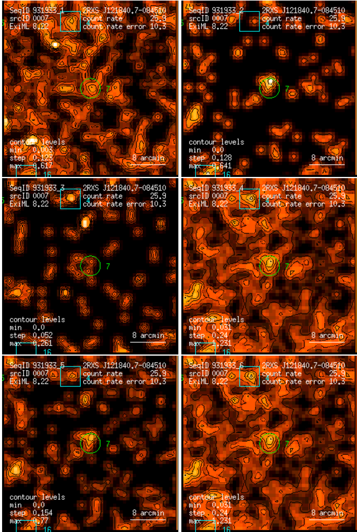
Figure 7: RASS 931933: detection 0007: band rate images, Gaussian filter: (1) PSPC channels 11 – 41, (2) 52 – 90, (3) 91 – 201, (4) 11 – 235, (5) 52 – 201, (6) 11 – 201. Broad band rates in counts/ks. Band rate contour levels in counts/ks/arcmin 2 .
