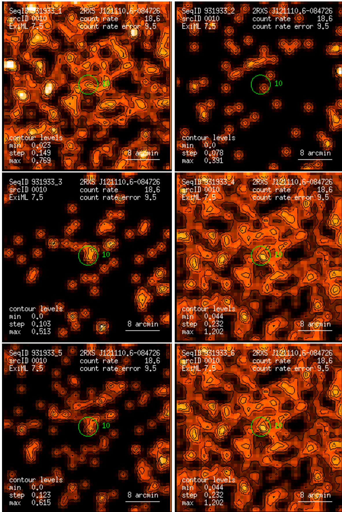
Figure 10: RASS 931933: detection 0010: band rate images, Gaussian filter: (1) PSPC channels 11 – 41, (2) 52 – 90, (3) 91 – 201, (4) 11 – 235, (5) 52 – 201, (6) 11 – 201. Broad band rates in counts/ks. Band rate contour levels in counts/ks/arcmin 2 .
