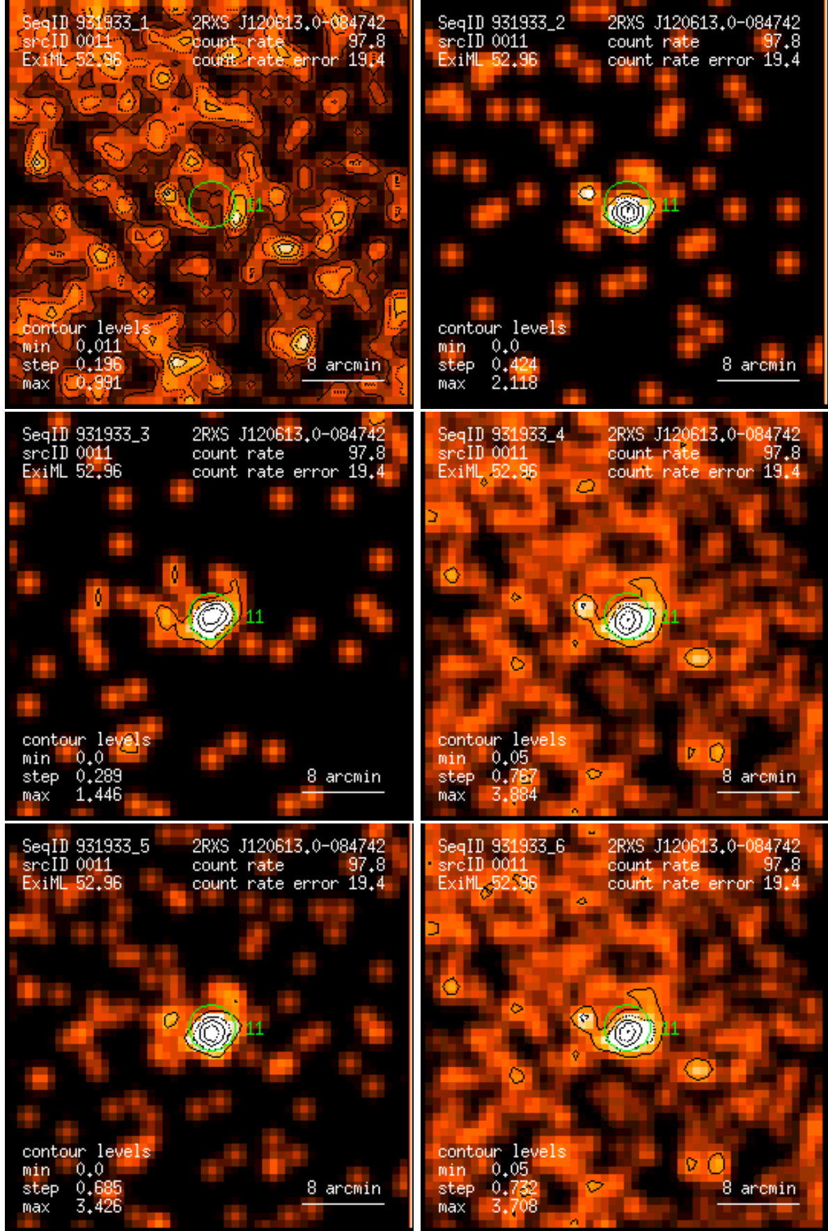
Figure 11: RASS 931933: detection 0011: band rate images, Gaussian filter: (1) PSPC channels 11 – 41, (2) 52 – 90, (3) 91 – 201, (4) 11 – 235, (5) 52 – 201, (6) 11 – 201. Broad band rates in counts/ks. Band rate contour levels in counts/ks/arcmin 2 .
