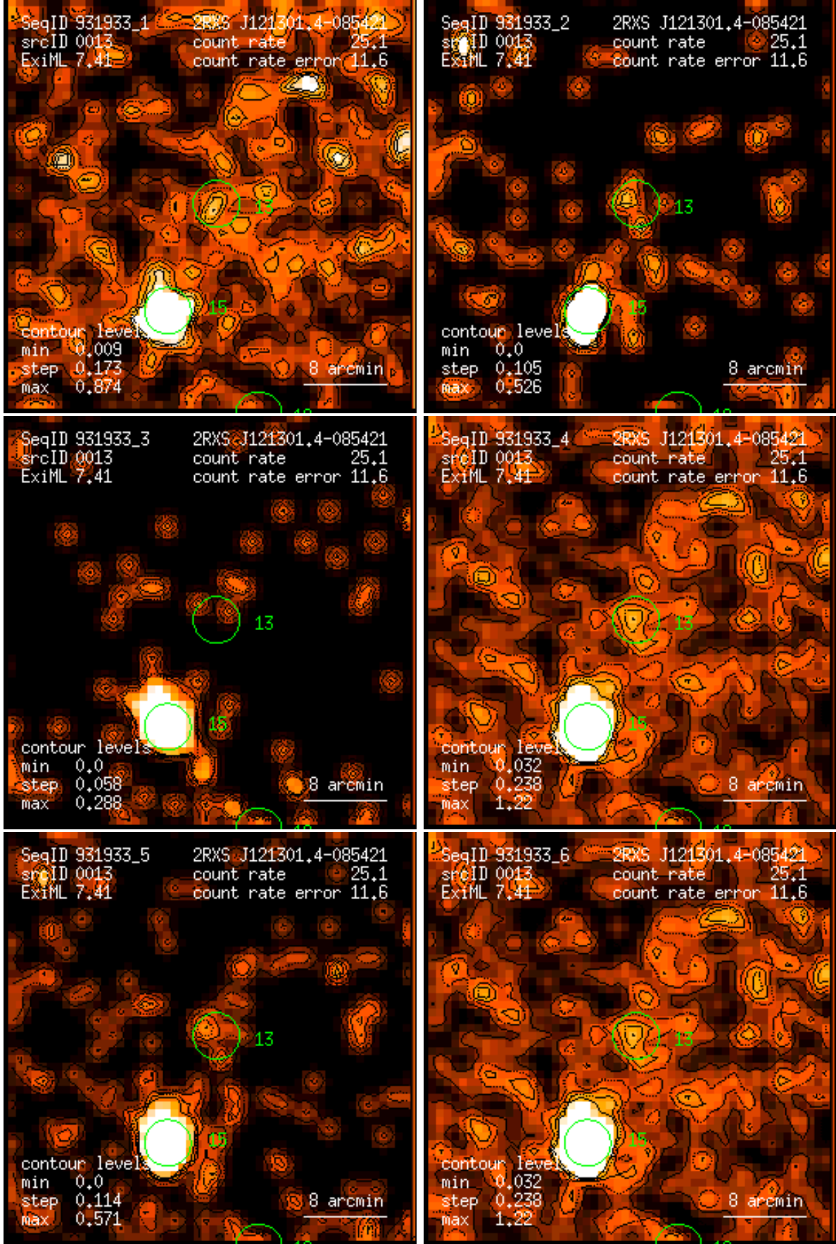
Figure 13: RASS 931933: detection 0013: band rate images, Gaussian filter: (1) PSPC channels 11 – 41, (2) 52 – 90, (3) 91 – 201, (4) 11 – 235, (5) 52 – 201, (6) 11 – 201. Broad band rates in counts/ks. Band rate contour levels in counts/ks/arcmin 2 .
