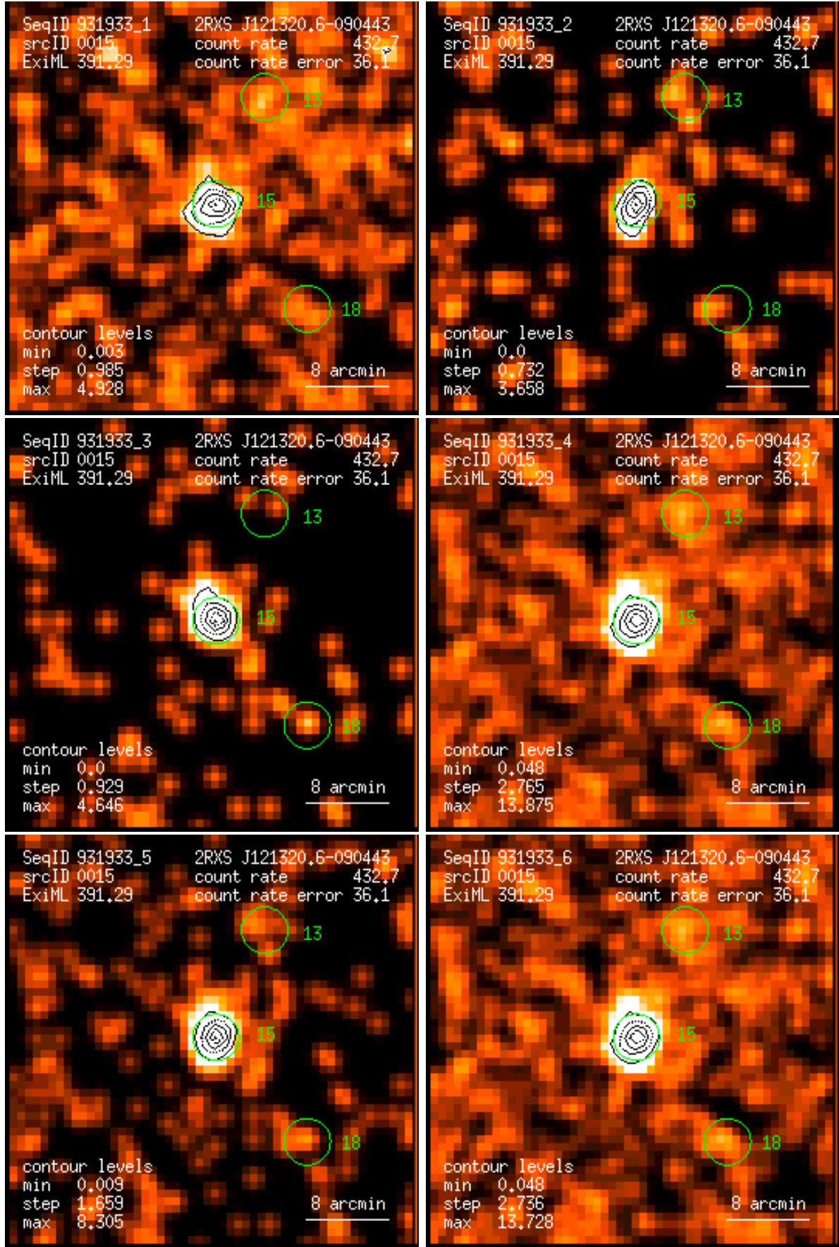
Figure 15: RASS 931933: detection 0015: band rate images, Gaussian filter: (1) PSPC channels 11 – 41, (2) 52 – 90, (3) 91 – 201, (4) 11 – 235, (5) 52 – 201, (6) 11 – 201. Broad band rates in counts/ks. Band rate contour levels in counts/ks/arcmin 2 .
