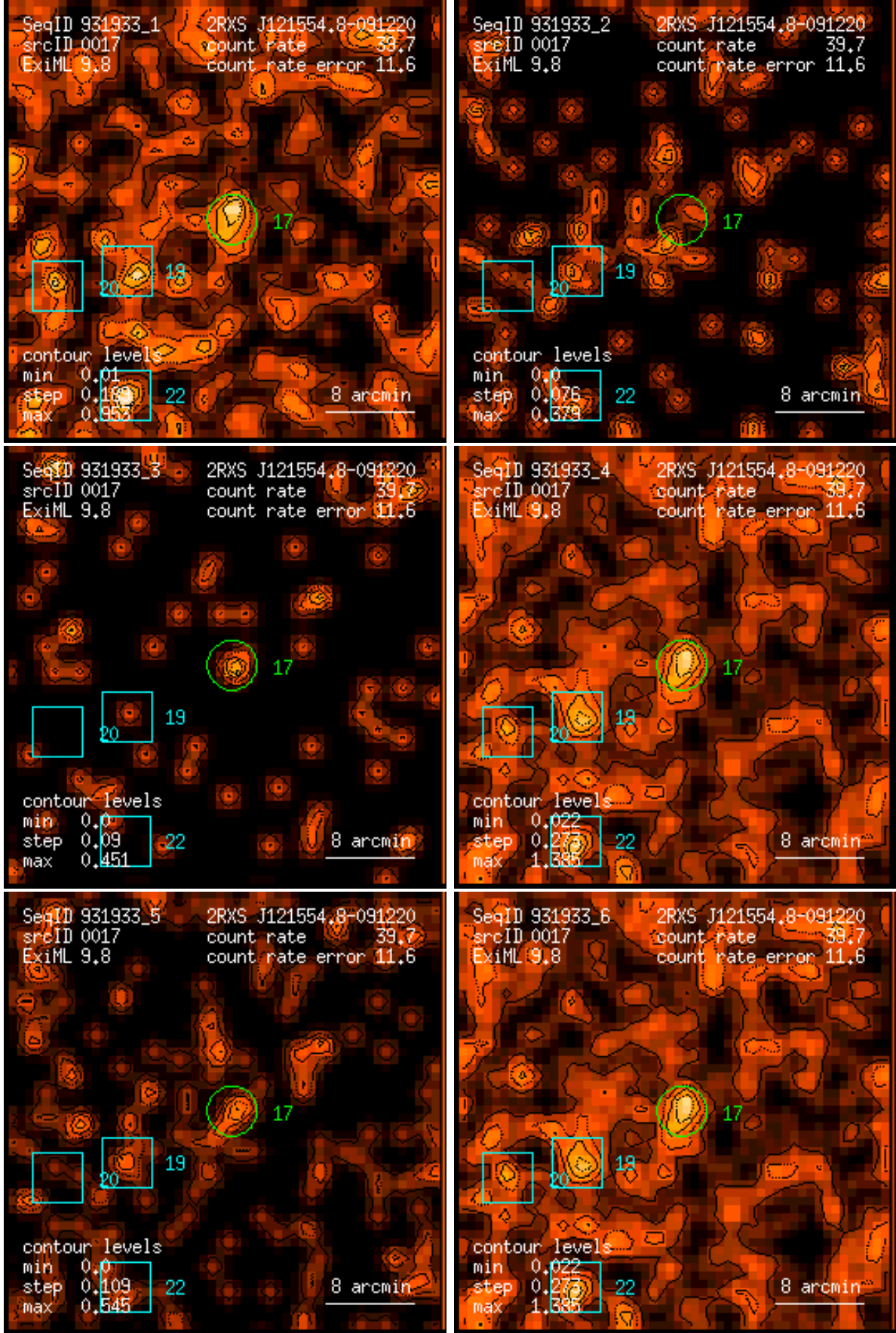
Figure 17: RASS 931933: detection 0017: band rate images, Gaussian filter: (1) PSPC channels 11 – 41, (2) 52 – 90, (3) 91 – 201, (4) 11 – 235, (5) 52 – 201, (6) 11 – 201. Broad band rates in counts/ks. Band rate contour levels in counts/ks/arcmin 2 .
