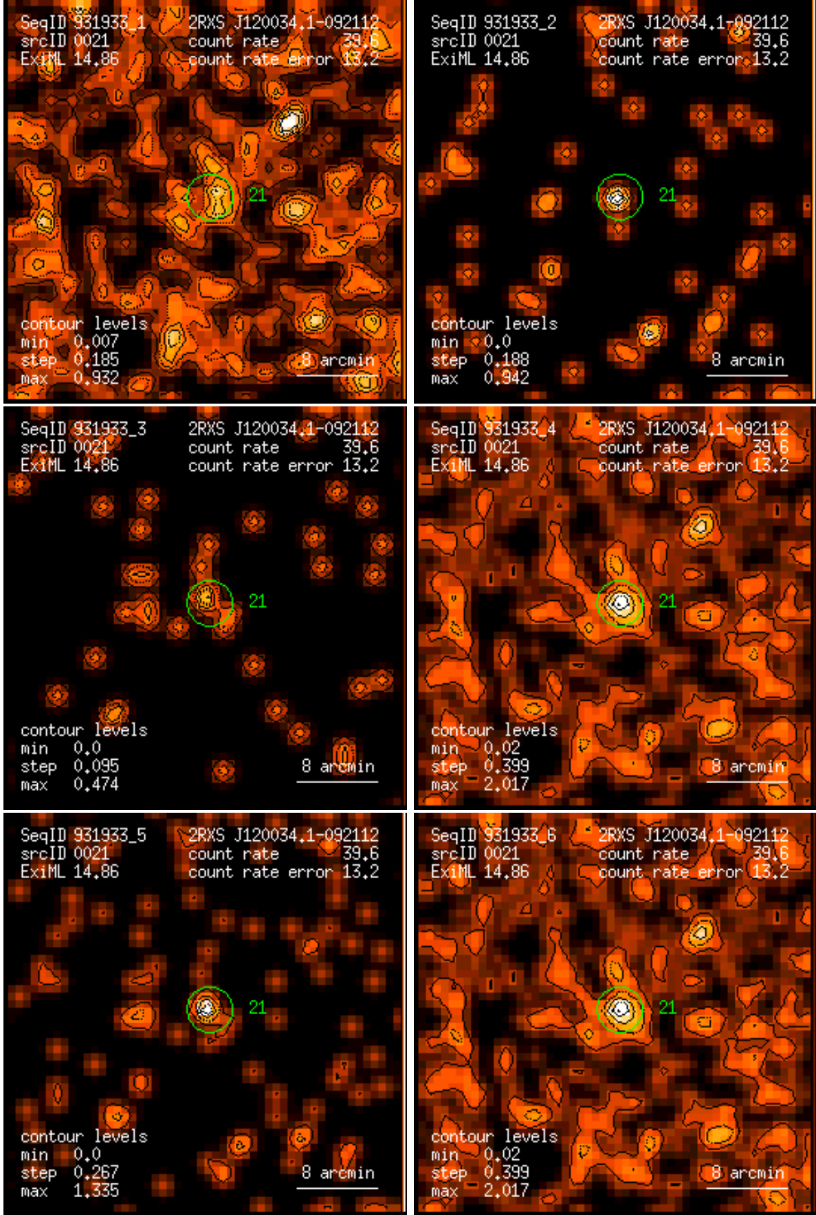
Figure 21: RASS 931933: detection 0021: band rate images, Gaussian filter: (1) PSPC channels 11 – 41, (2) 52 – 90, (3) 91 – 201, (4) 11 – 235, (5) 52 – 201, (6) 11 – 201. Broad band rates in counts/ks. Band rate contour levels in counts/ks/arcmin 2 .
