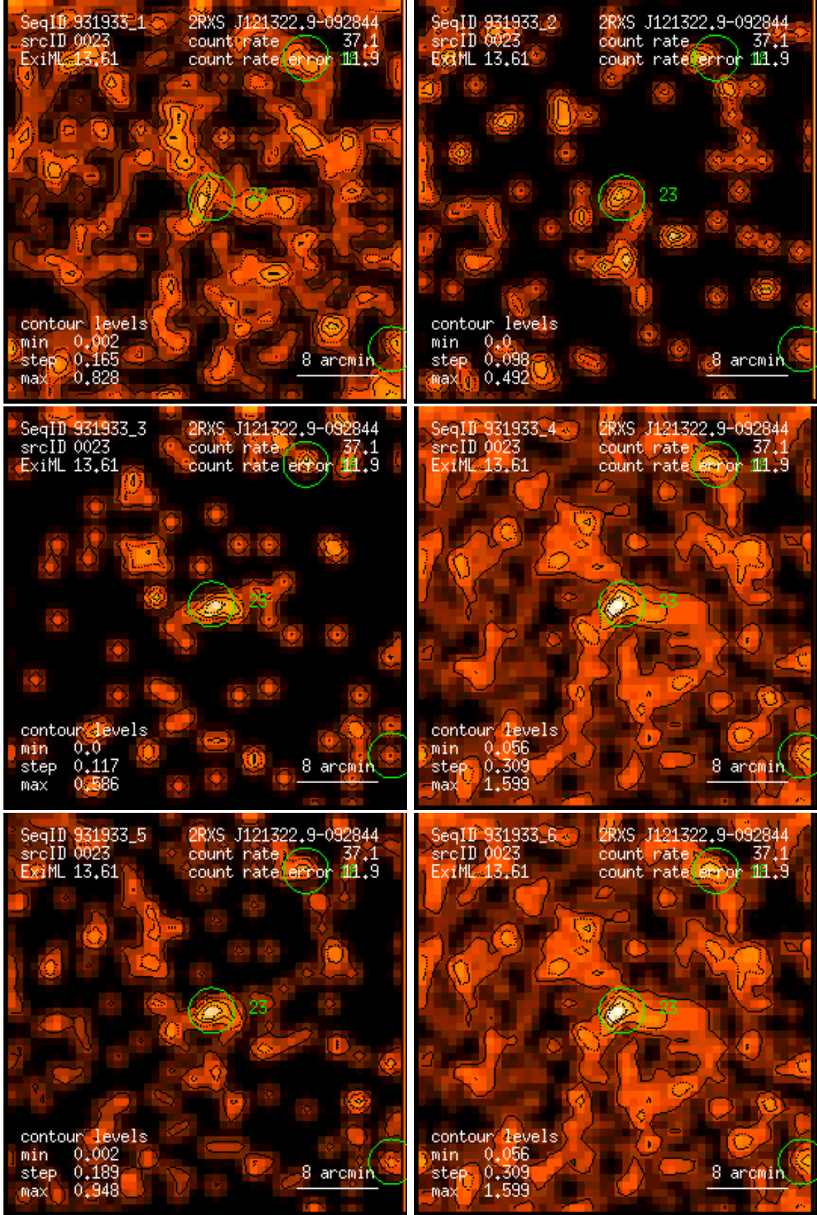
Figure 23: RASS 931933: detection 0023: band rate images, Gaussian filter: (1) PSPC channels 11 – 41, (2) 52 – 90, (3) 91 – 201, (4) 11 – 235, (5) 52 – 201, (6) 11 – 201. Broad band rates in counts/ks. Band rate contour levels in counts/ks/arcmin 2 .
