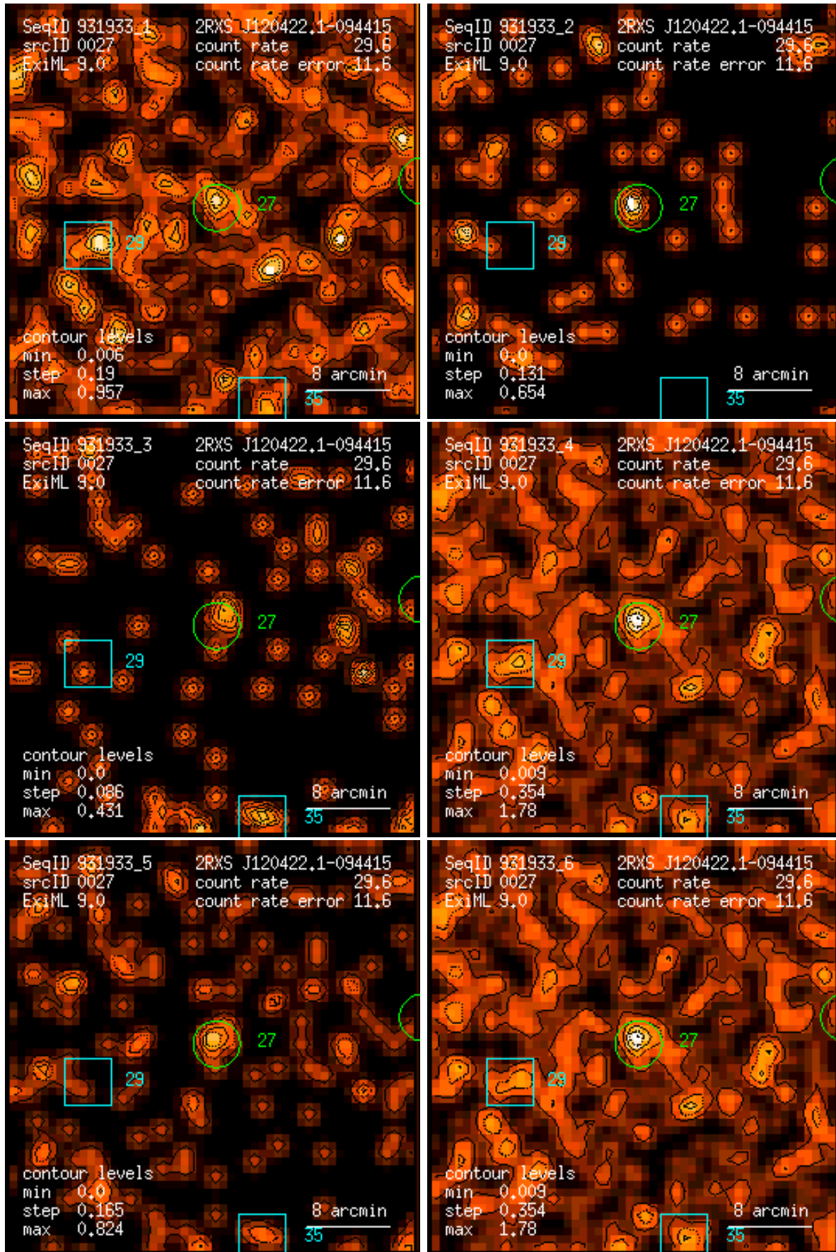
Figure 27: RASS 931933: detection 0027: band rate images, Gaussian filter: (1) PSPC channels 11 – 41, (2) 52 – 90, (3) 91 – 201, (4) 11 – 235, (5) 52 – 201, (6) 11 – 201. Broad band rates in counts/ks. Band rate contour levels in counts/ks/arcmin 2 .
