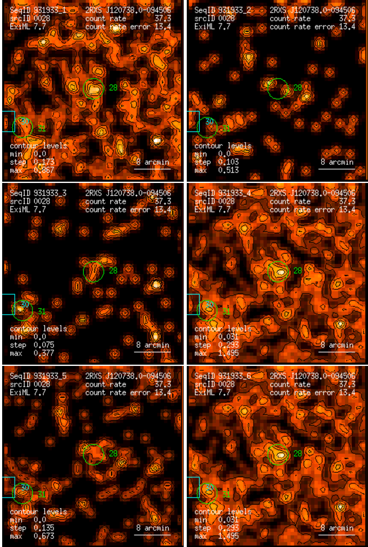
Figure 28: RASS 931933: detection 0028: band rate images, Gaussian filter: (1) PSPC channels 11 – 41, (2) 52 – 90, (3) 91 – 201, (4) 11 – 235, (5) 52 – 201, (6) 11 – 201. Broad band rates in counts/ks. Band rate contour levels in counts/ks/arcmin 2 .
