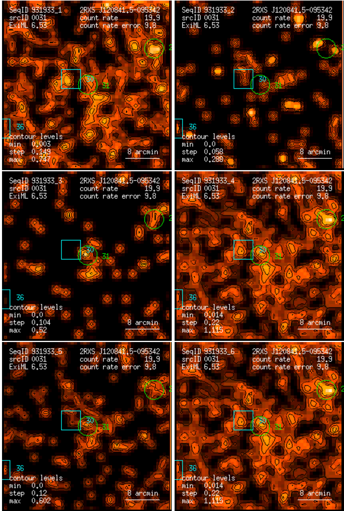
Figure 31: RASS 931933: detection 0031: band rate images, Gaussian filter: (1) PSPC channels 11 – 41, (2) 52 – 90, (3) 91 – 201, (4) 11 – 235, (5) 52 – 201, (6) 11 – 201. Broad band rates in counts/ks. Band rate contour levels in counts/ks/arcmin 2 .
