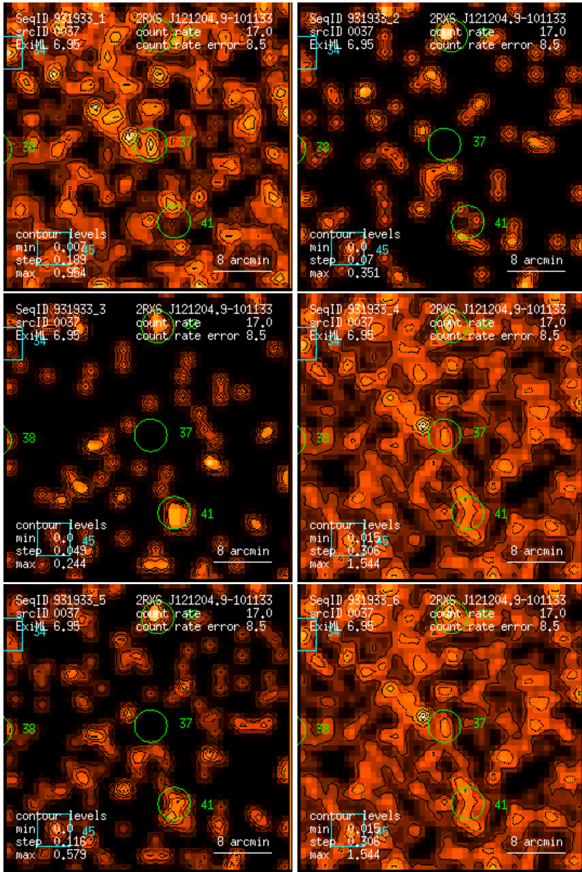
Figure 37: RASS 931933: detection 0037: band rate images, Gaussian filter: (1) PSPC channels 11 – 41, (2) 52 – 90, (3) 91 – 201, (4) 11 – 235, (5) 52 – 201, (6) 11 – 201. Broad band rates in counts/ks. Band rate contour levels in counts/ks/arcmin 2 .
