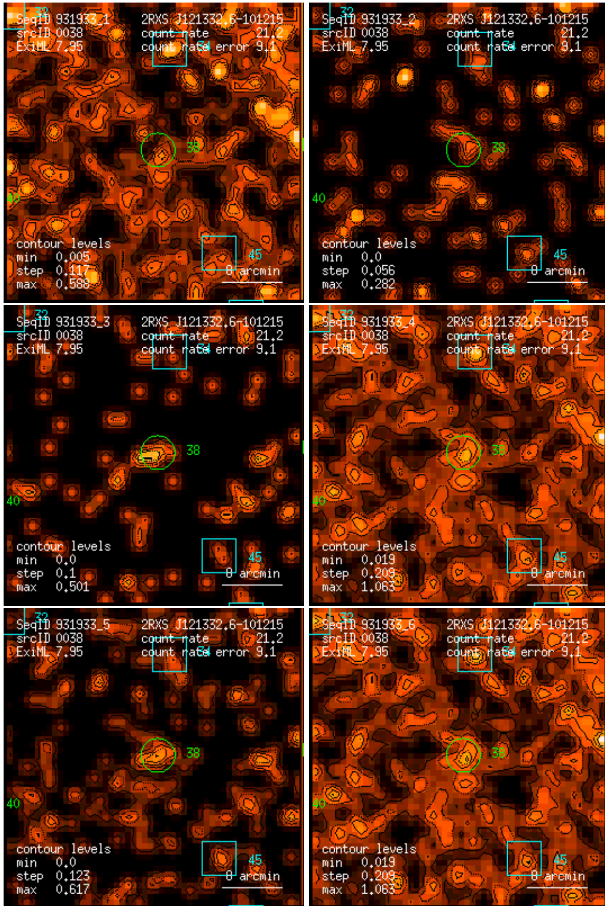
Figure 38: RASS 931933: detection 0038: band rate images, Gaussian filter: (1) PSPC channels 11 – 41, (2) 52 – 90, (3) 91 – 201, (4) 11 – 235, (5) 52 – 201, (6) 11 – 201. Broad band rates in counts/ks. Band rate contour levels in counts/ks/arcmin 2 .
