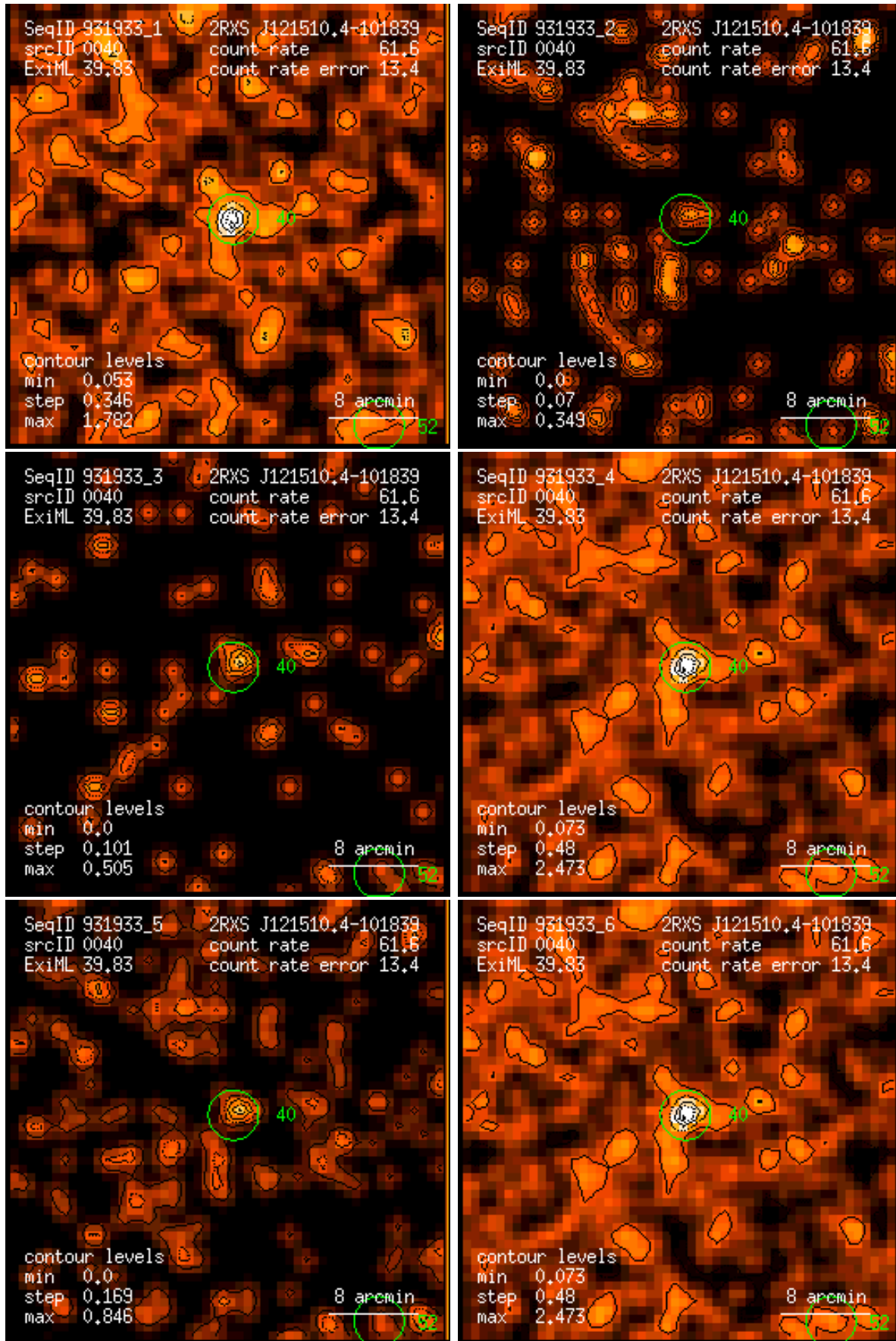
Figure 40: RASS 931933: detection 0040: band rate images, Gaussian filter: (1) PSPC channels 11 – 41, (2) 52 – 90, (3) 91 – 201, (4) 11 – 235, (5) 52 – 201, (6) 11 – 201. Broad band rates in counts/ks. Band rate contour levels in counts/ks/arcmin 2 .
