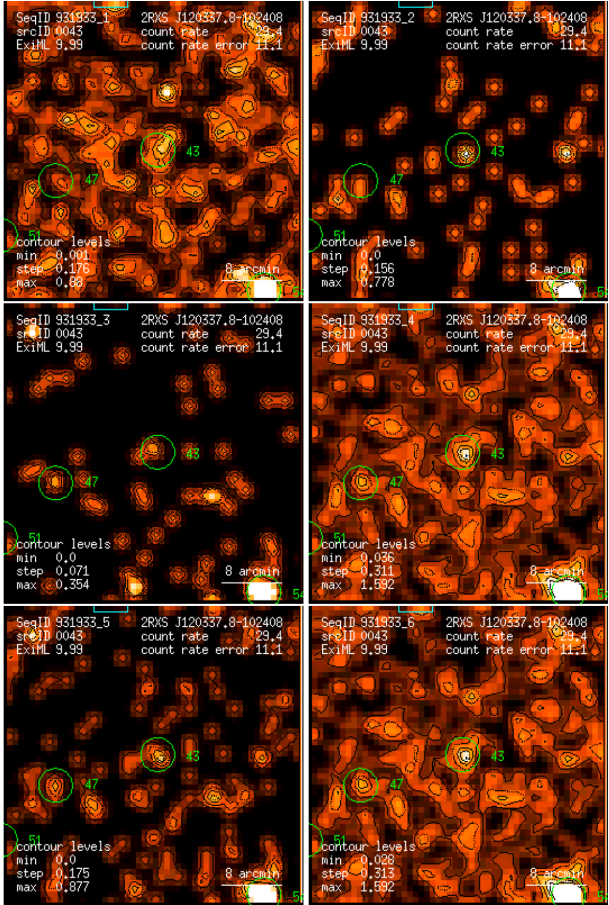
Figure 43: RASS 931933: detection 0043: band rate images, Gaussian filter: (1) PSPC channels 11 – 41, (2) 52 – 90, (3) 91 – 201, (4) 11 – 235, (5) 52 – 201, (6) 11 – 201. Broad band rates in counts/ks. Band rate contour levels in counts/ks/arcmin 2 .
