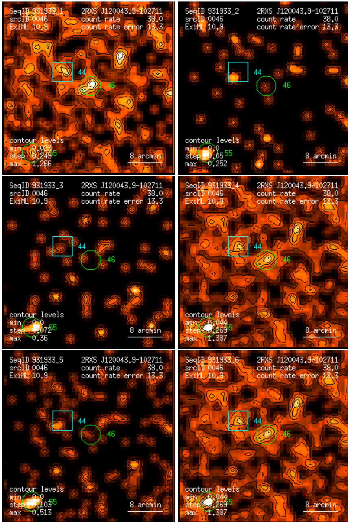
Figure 46: RASS 931933: detection 0046: band rate images, Gaussian filter: (1) PSPC channels 11 – 41, (2) 52 – 90, (3) 91 – 201, (4) 11 – 235, (5) 52 – 201, (6) 11 – 201. Broad band rates in counts/ks. Band rate contour levels in counts/ks/arcmin 2 .
