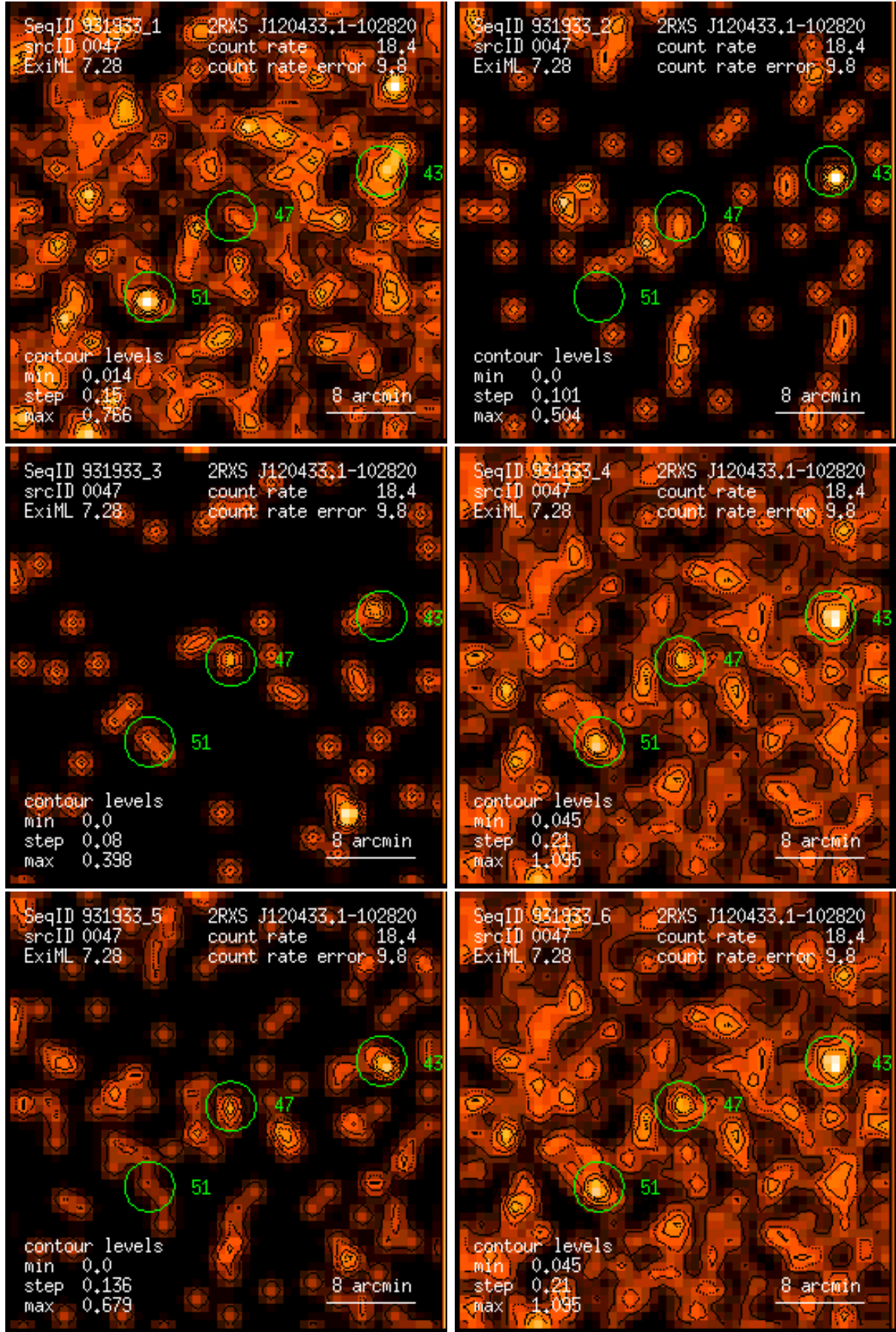
Figure 47: RASS 931933: detection 0047: band rate images, Gaussian filter: (1) PSPC channels 11 – 41, (2) 52 – 90, (3) 91 – 201, (4) 11 – 235, (5) 52 – 201, (6) 11 – 201. Broad band rates in counts/ks. Band rate contour levels in counts/ks/arcmin 2 .
