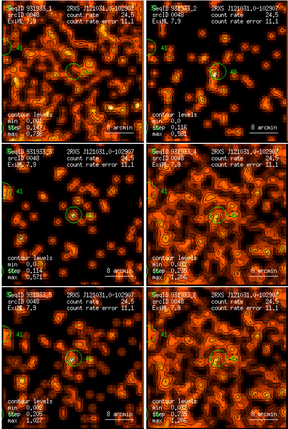
Figure 48: RASS 931933: detection 0048: band rate images, Gaussian filter: (1) PSPC channels 11 – 41, (2) 52 – 90, (3) 91 – 201, (4) 11 – 235, (5) 52 – 201, (6) 11 – 201. Broad band rates in counts/ks. Band rate contour levels in counts/ks/arcmin 2 .
