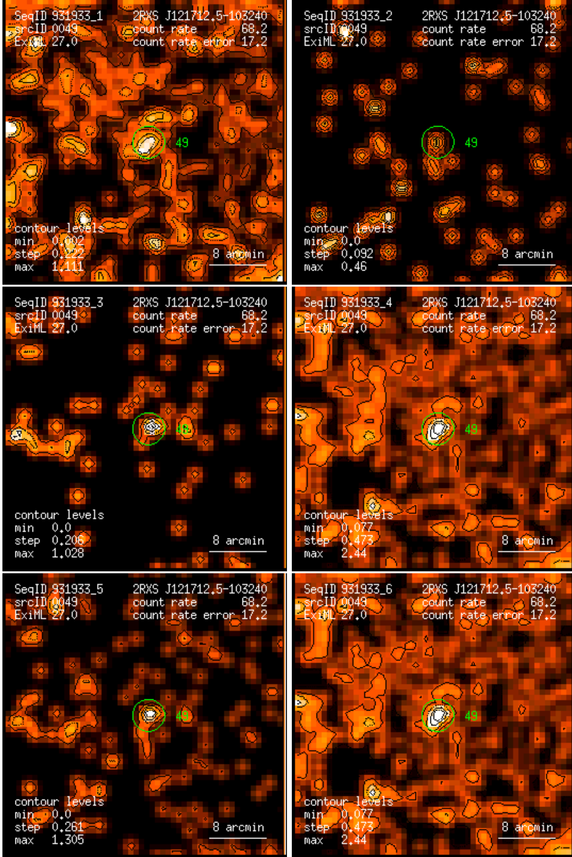
Figure 49: RASS 931933: detection 0049: band rate images, Gaussian filter: (1) PSPC channels 11 – 41, (2) 52 – 90, (3) 91 – 201, (4) 11 – 235, (5) 52 – 201, (6) 11 – 201. Broad band rates in counts/ks. Band rate contour levels in counts/ks/arcmin 2 .
