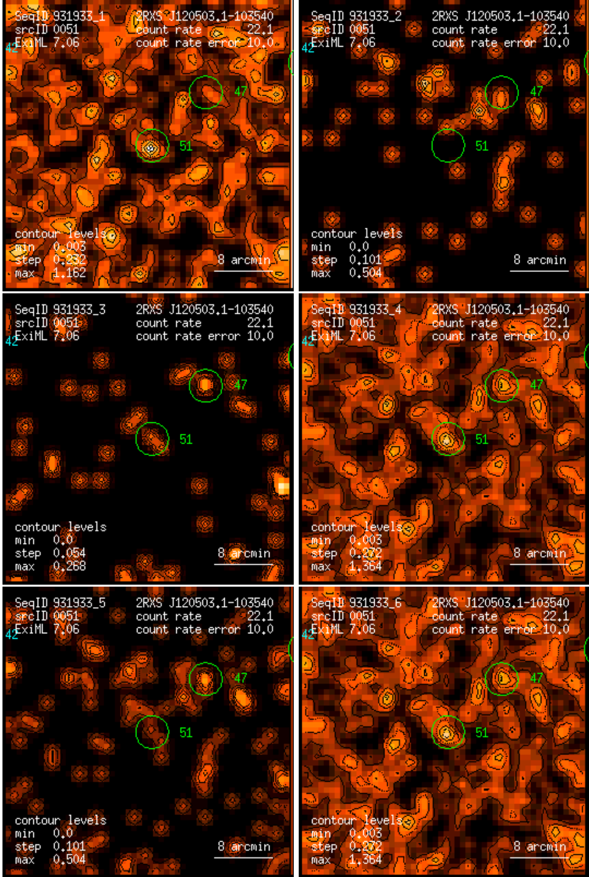
Figure 51: RASS 931933: detection 0051: band rate images, Gaussian filter: (1) PSPC channels 11 – 41, (2) 52 – 90, (3) 91 – 201, (4) 11 – 235, (5) 52 – 201, (6) 11 – 201. Broad band rates in counts/ks. Band rate contour levels in counts/ks/arcmin 2 .
