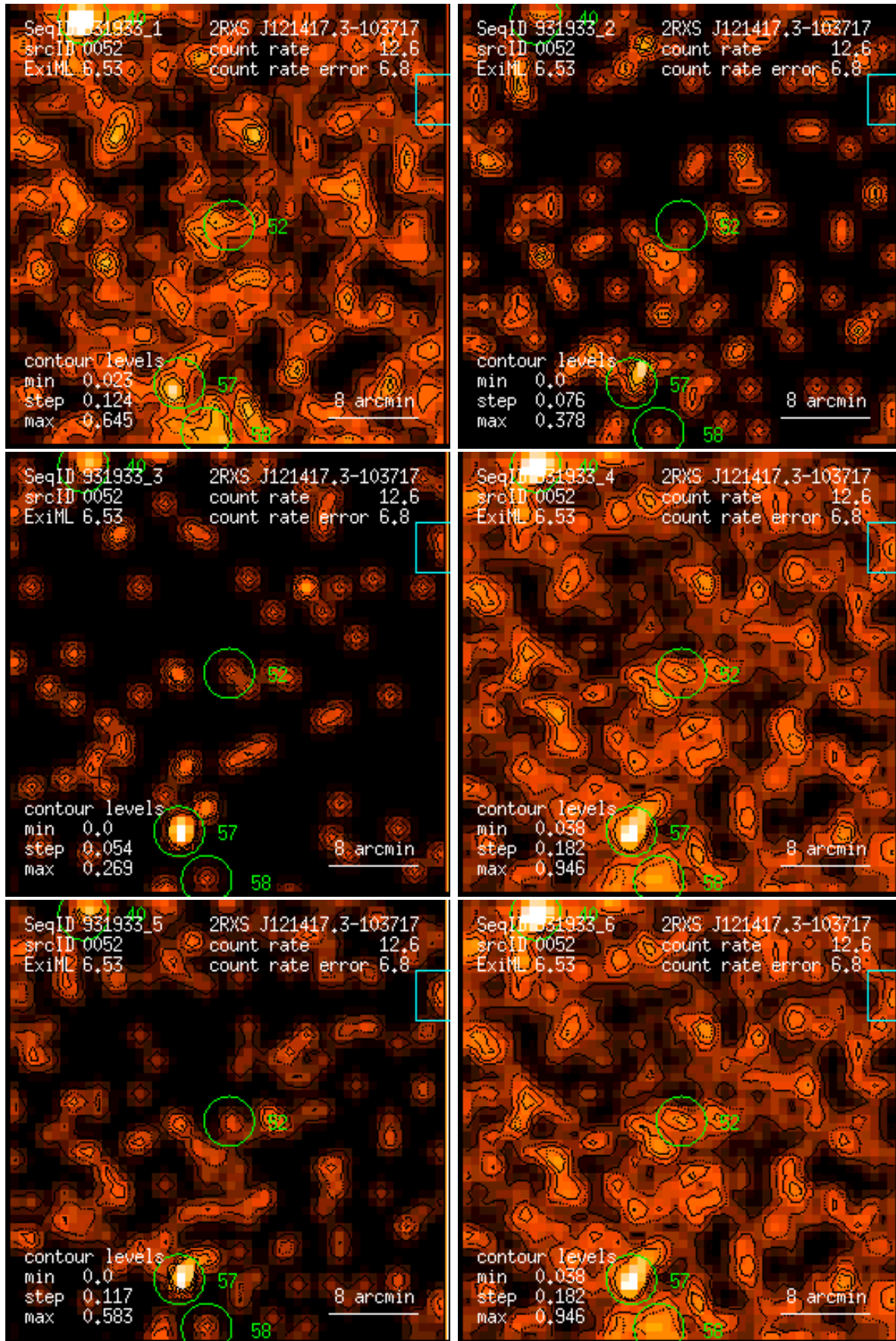
Figure 52: RASS 931933: detection 0052: band rate images, Gaussian filter: (1) PSPC channels 11 – 41, (2) 52 – 90, (3) 91 – 201, (4) 11 – 235, (5) 52 – 201, (6) 11 – 201. Broad band rates in counts/ks. Band rate contour levels in counts/ks/arcmin 2 .
