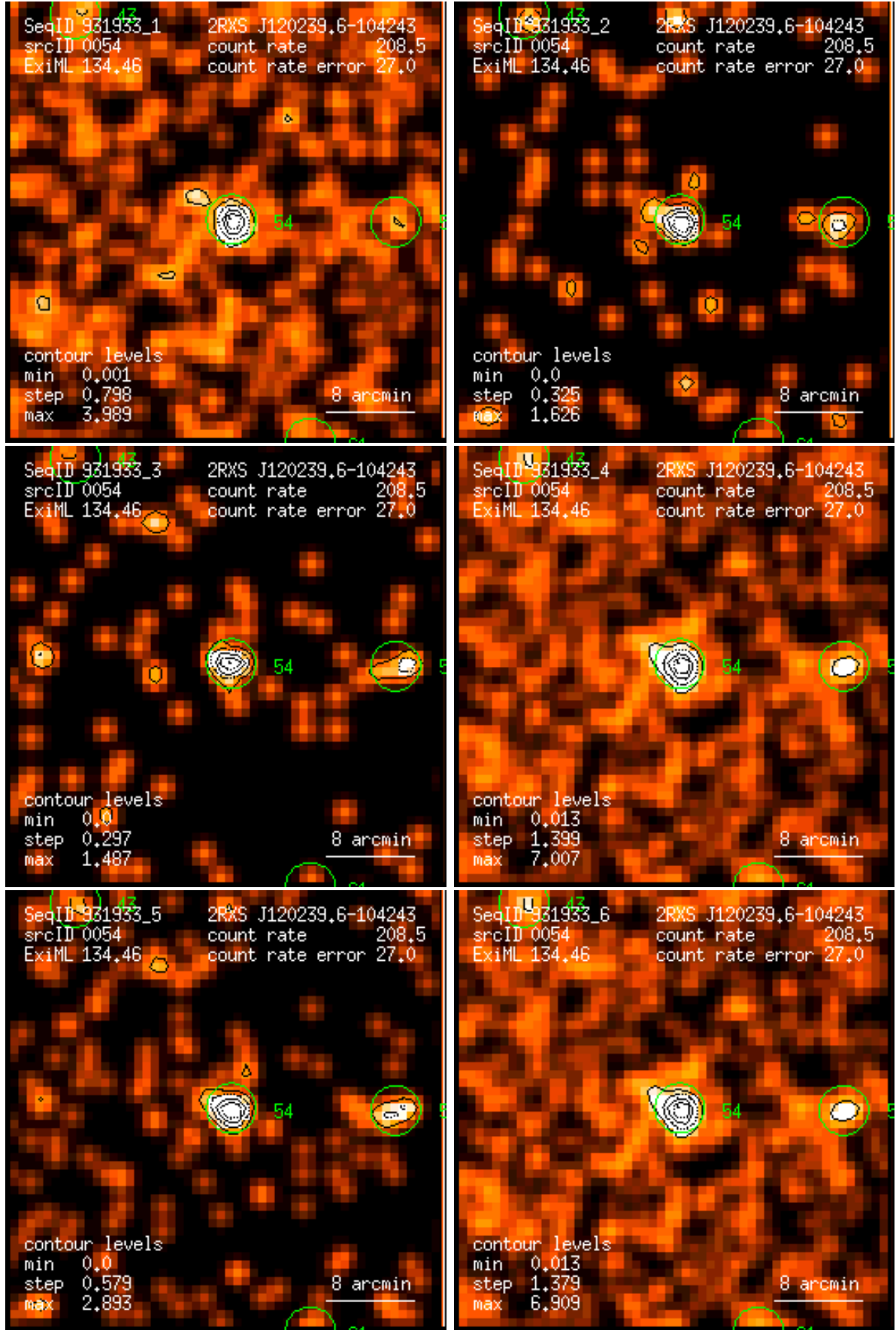
Figure 54: RASS 931933: detection 0054: band rate images, Gaussian filter: (1) PSPC channels 11 – 41, (2) 52 – 90, (3) 91 – 201, (4) 11 – 235, (5) 52 – 201, (6) 11 – 201. Broad band rates in counts/ks. Band rate contour levels in counts/ks/arcmin 2 .
