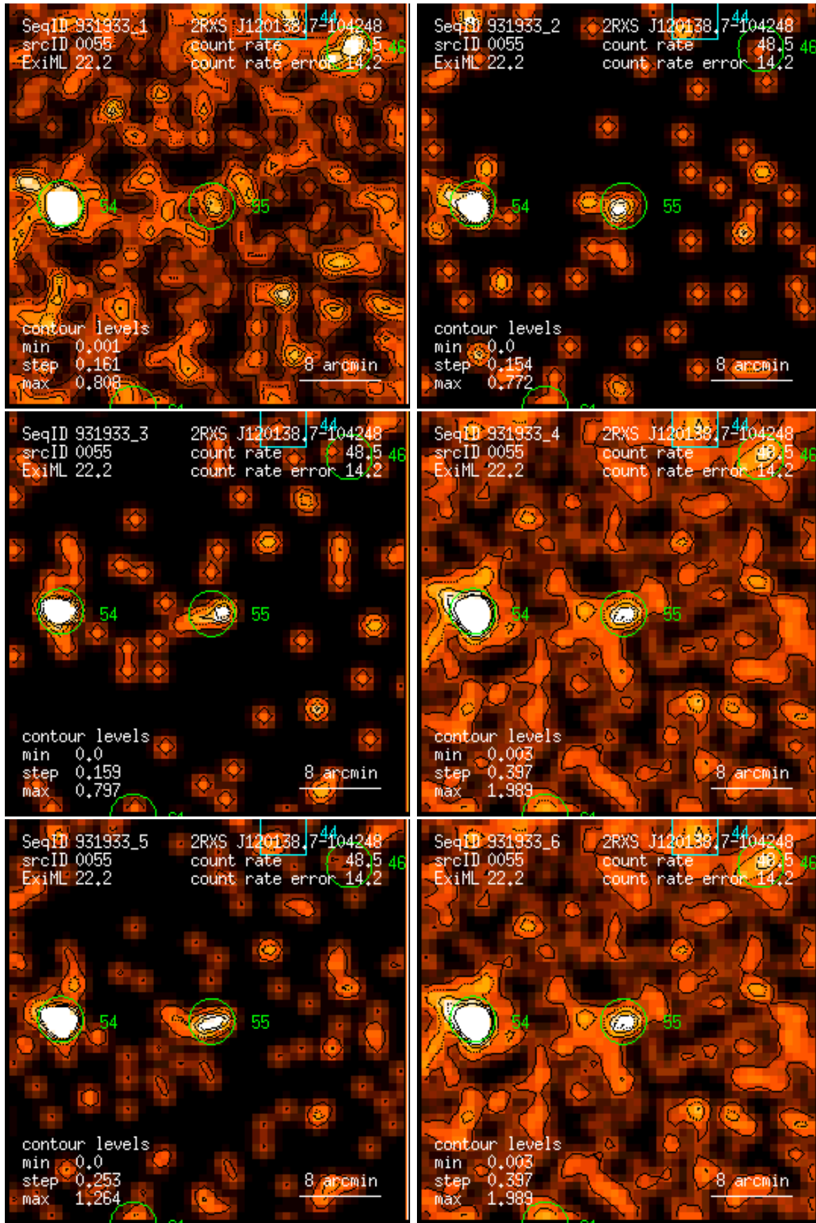
Figure 55: RASS 931933: detection 0055: band rate images, Gaussian filter: (1) PSPC channels 11 – 41, (2) 52 – 90, (3) 91 – 201, (4) 11 – 235, (5) 52 – 201, (6) 11 – 201. Broad band rates in counts/ks. Band rate contour levels in counts/ks/arcmin 2 .
