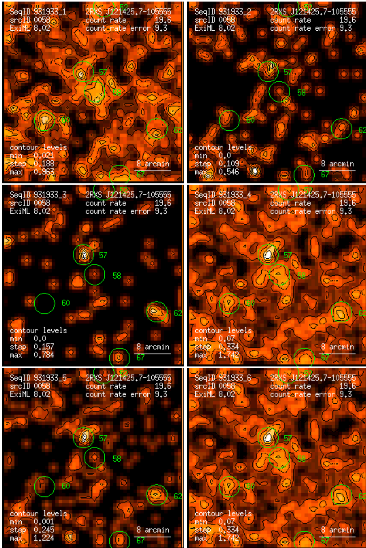
Figure 58: RASS 931933: detection 0058: band rate images, Gaussian filter: (1) PSPC channels 11 – 41, (2) 52 – 90, (3) 91 – 201, (4) 11 – 235, (5) 52 – 201, (6) 11 – 201. Broad band rates in counts/ks. Band rate contour levels in counts/ks/arcmin 2 .
