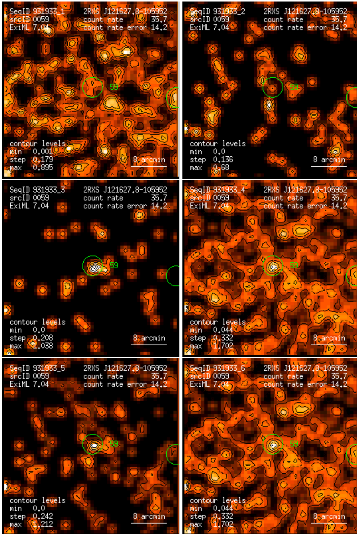
Figure 59: RASS 931933: detection 0059: band rate images, Gaussian filter: (1) PSPC channels 11 – 41, (2) 52 – 90, (3) 91 – 201, (4) 11 – 235, (5) 52 – 201, (6) 11 – 201. Broad band rates in counts/ks. Band rate contour levels in counts/ks/arcmin 2 .
