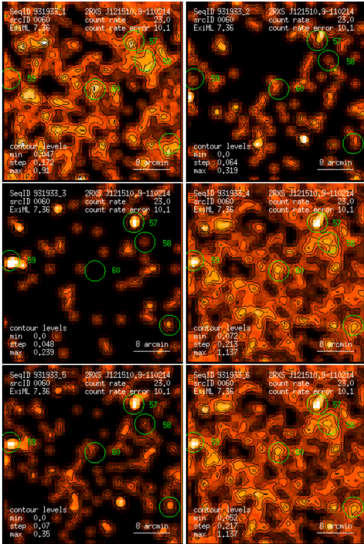
Figure 60: RASS 931933: detection 0060: band rate images, Gaussian filter: (1) PSPC channels 11 – 41, (2) 52 – 90, (3) 91 – 201, (4) 11 – 235, (5) 52 – 201, (6) 11 – 201. Broad band rates in counts/ks. Band rate contour levels in counts/ks/arcmin 2 .
