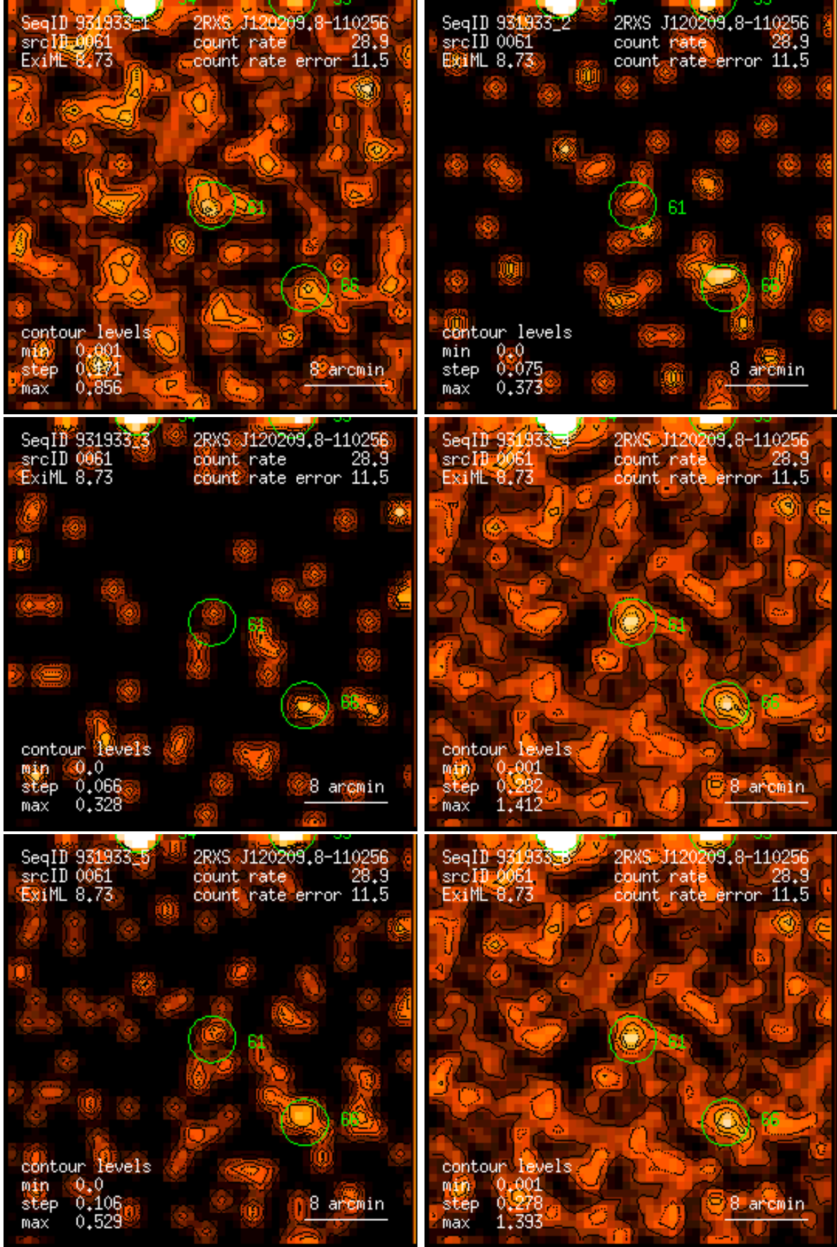
Figure 61: RASS 931933: detection 0061: band rate images, Gaussian filter: (1) PSPC channels 11 – 41, (2) 52 – 90, (3) 91 – 201, (4) 11 – 235, (5) 52 – 201, (6) 11 – 201. Broad band rates in counts/ks. Band rate contour levels in counts/ks/arcmin 2 .
